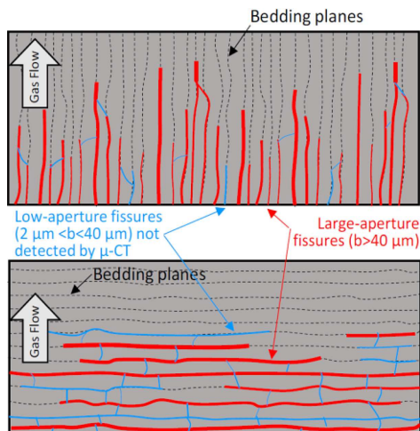
Fig. 2. Schematic representation of expected gas flow at different orientations of bedding planes: parallel to flow (top) and orthogonal to flow (bottom). Dashed thin lines represent bedding planes. Solid lines depict the volume occupied by gas: apertures larger than 40\ \mu\text{m} and detected by \mu\text{-CT} (in red); and apertures between 2 and 40\ \mu\text{m} detected by MIP but not by \mu\text{-CT} (in blue) [12].
