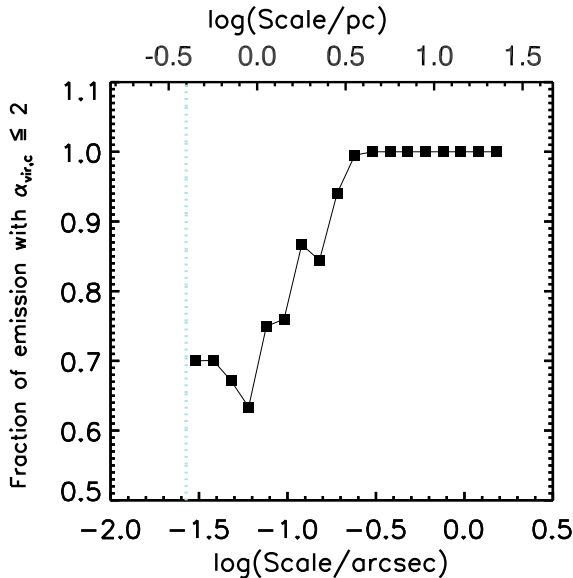
Figure 8. Fraction of emission originating from gravitationally bound (i.e. self-gravitating) structures ( \alpha_{\text{vir},c} \leq \alpha_{\text{vir},c,\text{crit}} = 2 ) as a function of the structures’ spatial scales in NGC 404. The fraction grows with scale and saturates at 1 at scales \gtrsim 3 pc. The blue vertical dotted line indicates our spatial resolution limit of 0.027 arcsec or 0.40 pc (i.e. half the synthesized beam).
