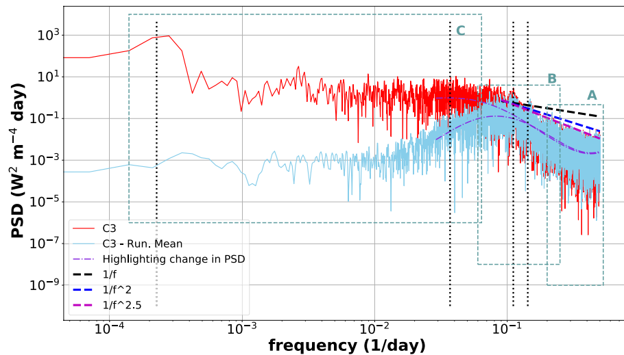
Figure C3. Power Spectrum Density (PSD) of total solar irradiance (TSI) C3 (Fröhlich, 2006) with and without partially removing the solar cycle via a running mean (with a 5-day window). Boxes A, B and C refer to the different sections of the PSD. The dash-dotted lines are the various power-law models when varying the exponent. The vertical dotted lines (black) mark the frequencies at 11.5 years, 27, 9 and 7 days. The purple dash-dotted lines highlight the change of power in box C before and after removing the solar cycle.
