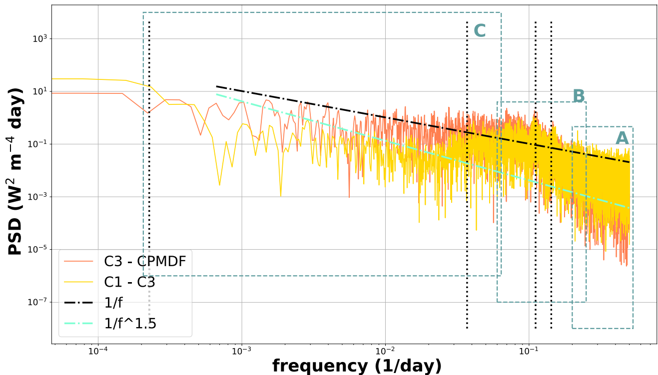
Figure 4. Power Spectrum Density of the difference of composite time series including C3 - Composite PMOD- Data Fusion (CPMDF), C1 - C3 . The vertical dotted lines (black) mark the frequencies at 11.5 years, 27, 9 and 7 days (left to right).
