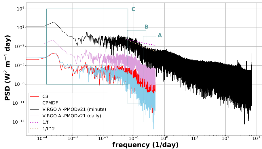
Figure C4. Power Spectrum Density (PSD) of various products: VIRGO/SOHO with degradation correction (VIRGO-A) from PMO6v21 with 1-min and daily sampling rate. C3 is the total solar irradiance (TSI) composite produced by Fröhlich (2006). Composite PMOD-Data Fusion is our new TSI composite including the wavelet filter. Note that for clarity the different spectra have been rescaled by multiplying them by -6 , -6 , -4 and -8.5 \text{ W}^2 \text{ m}^{-4} \text{ day} following the order of the legends from the top. Boxes A, B and C refer to the different sections of the PSD. The dash lines are the various power-law models when varying the exponent (shown for context). The vertical dashed line emphasizes the 11.5 years peak.
