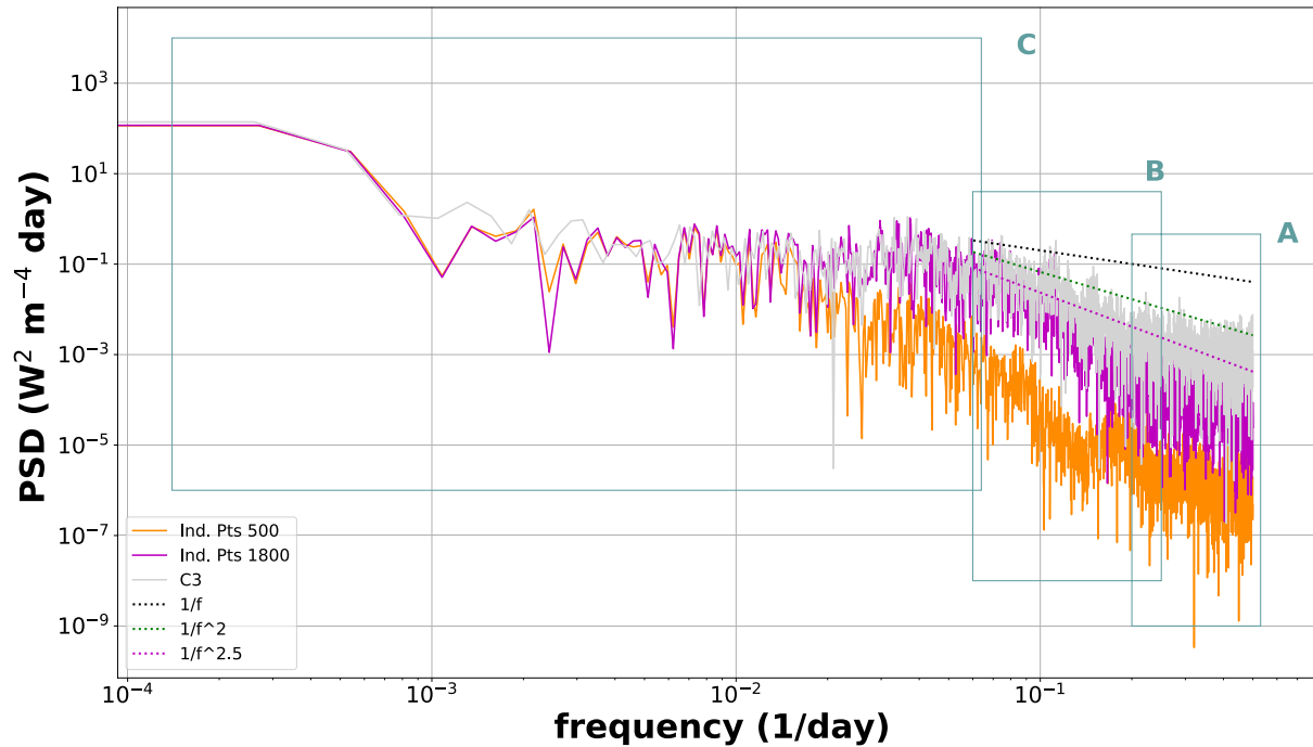
Figure C2. Power Spectrum Density (PSD) of total solar irradiance (TSI) C3 (Fröhlich, 2006) and the sub-time series in Box 8 fusing VIRGO/SOHO, ACRIM3/ACRIMSAT and TIM/SORCE using various numbers of inducing points (500, 1,800). Box A, B and C refer to the different sections of the PSD: A is centered on the high frequency (~3 days), which shows flattening of the PSD; B is the power-law which is mainly due to colored noise (correlations between 20 and 6 days) within the time series; C emphasizes the low frequency associated with the stochastic and deterministic parts of the solar cycle and long-term correlations, as well as instrumental artifacts. The dashed line is the power-law model when varying the exponent (shown for context).
