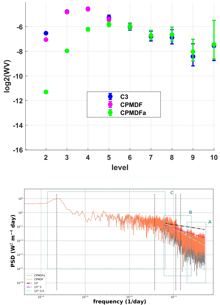
Figure B1. (top) Wavelet Variance (WV) decomposition of C3 (blue), CPMDFa (green) and the filtered time series (pink). The X-axis is the level of decomposition, whereas the Y-axis is the WV value on a log scale. (bottom) Effect of applying the wavelet filter in the frequency domain: without CPMDFa (gray) and with CPMDF (orange).
