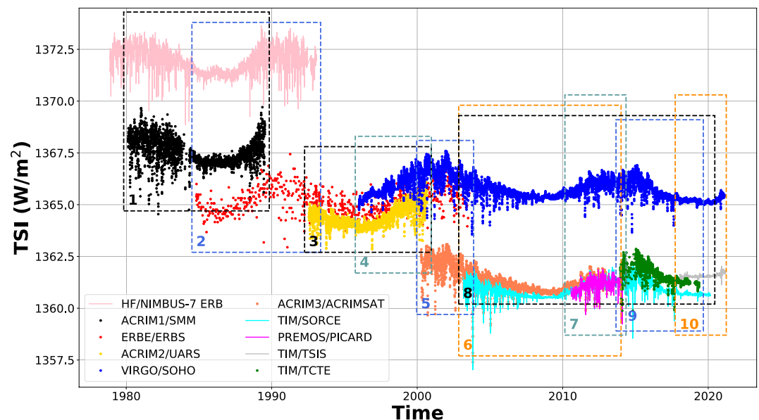
Figure 1. Various satellite missions which have conducted total solar irradiance (TSI) observations since the late 1970s. We perform the fusion using the observations included in each box (dash lines).
