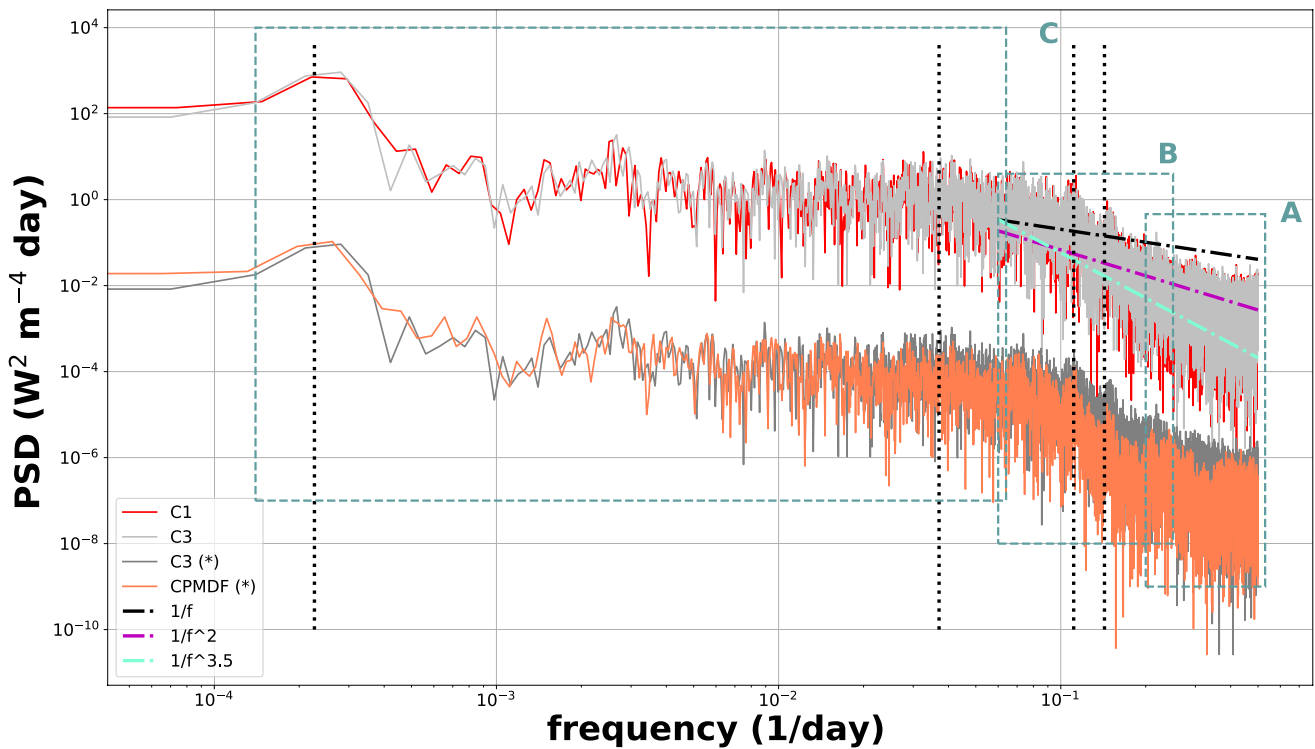
Figure 3. Power Spectrum Density (PSD) of total solar irradiance (TSI) CI (Dudok de Wit et al., 2017), C3 (Fröhlich, 2006), together with the new TSI composite produced with the current method Composite PMOD- Data Fusion (CPMDF) . The (*) means that the time series are shifted by rescaling the amplitude by -4 \text{ W}^2 \text{ m}^{-4} \text{ day} in the log-log plot. Box A , B and C refer to the different sections of the PSD: A is centered on the high frequency ( \sim 3 days) showing the flattening of the PSD; B is the power-law which is mainly due to colored noise (correlations between 20 and 6 days) within the time series; C emphasizes the low frequency associated with the stochastic and deterministic parts of the solar cycle and long-term correlations. The dashed lines are the various power-law models when varying the exponent, which are only shown for context. The vertical dotted lines (black) mark the frequencies at 11.5 years, 27, 9 and 7 days (left to right).
