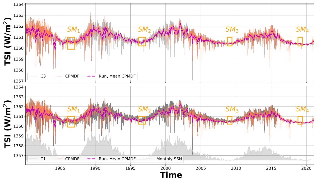
Figure 2. New composite Composite PMOD- Data Fusion (CPMDF, orange) based on merging 41 years of total solar irradiance (TSI) measurements. For comparison, C3 (Fröhlich, 2006) and C1 (Dudok de Wit et al., 2017) are also shown (gray line). A 30-day running mean of CPMDF is shown as a yellow/purple dashed line. The orange boxes are associated with the solar minima (SM) for each solar cycle described in Table 2. For context, the monthly sunspot number is also displayed.
