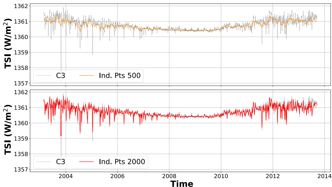
Figure C1. Time series of C3 (Fröhlich, 2006) and the sub-time series in Box 8 (see Figure 1) fusing VIRGO/SOHO, ACRIM3/ACRIMSAT and TIM/SORCE using various numbers of inducing points (500, 2,000). The sub-time series are aligned on C3 .
