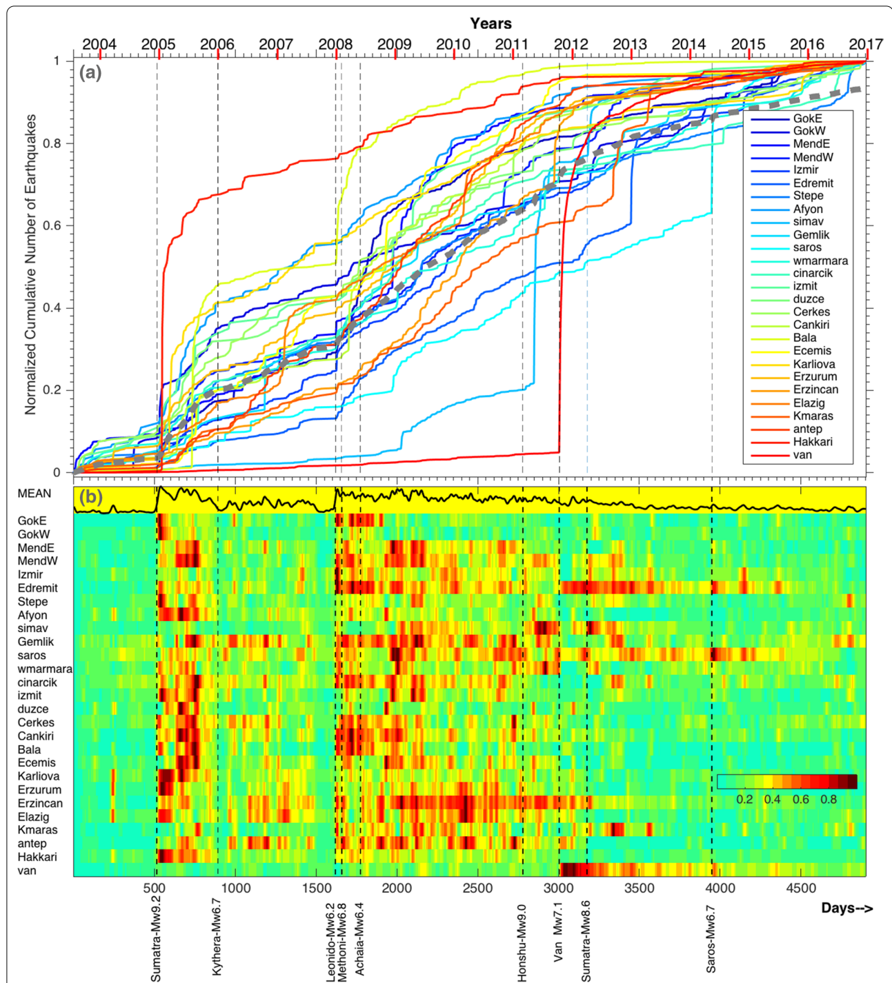
Fig. 2 Evolution of activity in the seismic clusters outlined in Fig. 1. a Cumulative number of earthquakes in each cluster. Time is measured from August 2003 and each curve is normalized to its final value. The dashed lines show the occurrence times of the large earthquakes discussed in the text. The gray dashed line shows the average of all clusters. The legend indicates the names of the clusters (see Fig. 1 for their locations). b Seismicity rates in each cluster. The upper black trace is the mean of the rates for all clusters. The names of the clusters are displayed on the left. The time series are displayed at increasing longitudes. The color scale shown on the lower right corner refers to the normalized cumulative number of earthquakes
