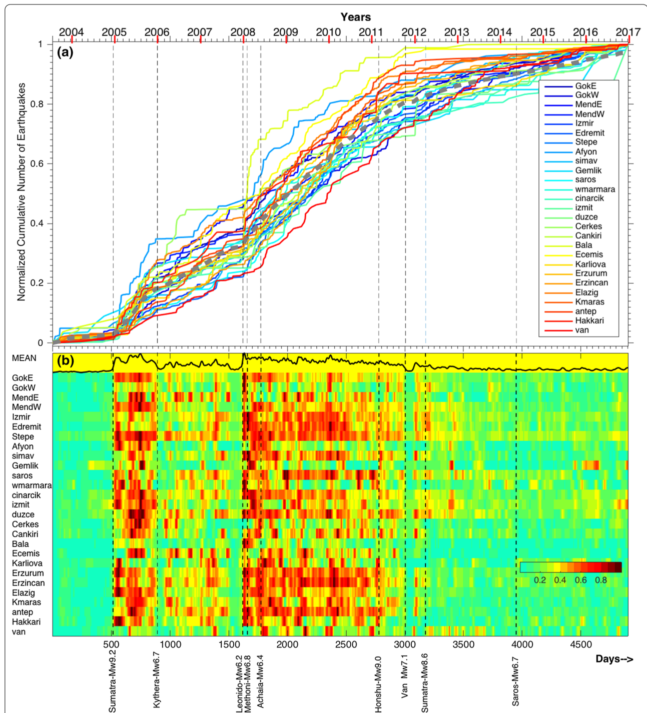
Fig. 4 a Evolution of cumulative number of earthquakes declustered using ETAS model of the seismic clusters shown in Fig. 1. Time is measured from August 2003 and each curve is normalized to its final value. The gray dashed line shows the average of all clusters. The black dashed lines show the occurrence times of giant earthquakes worldwide and of large regional earthquakes. The legend indicates the names of the clusters displayed in Fig. 1. b Seismicity rates of the clusters displayed in a . The upper black trace is the mean of the rates. The color scale shown on the lower right corner refers to the normalized cumulative number of earthquakes
