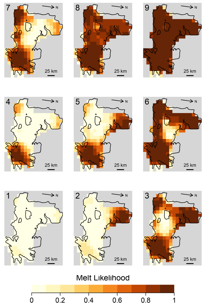
Figure 2. Result of the self-organising map, showing that nine representative melt patterns can describe the spatial variability in surface melt on the Shackleton Ice Shelf (2002/03–2020/21). Pixel values indicate how likely melt will be observed in a pixel on the days best described by the respective pattern; further explanation can be found in Sects. 3.2 and S1.
