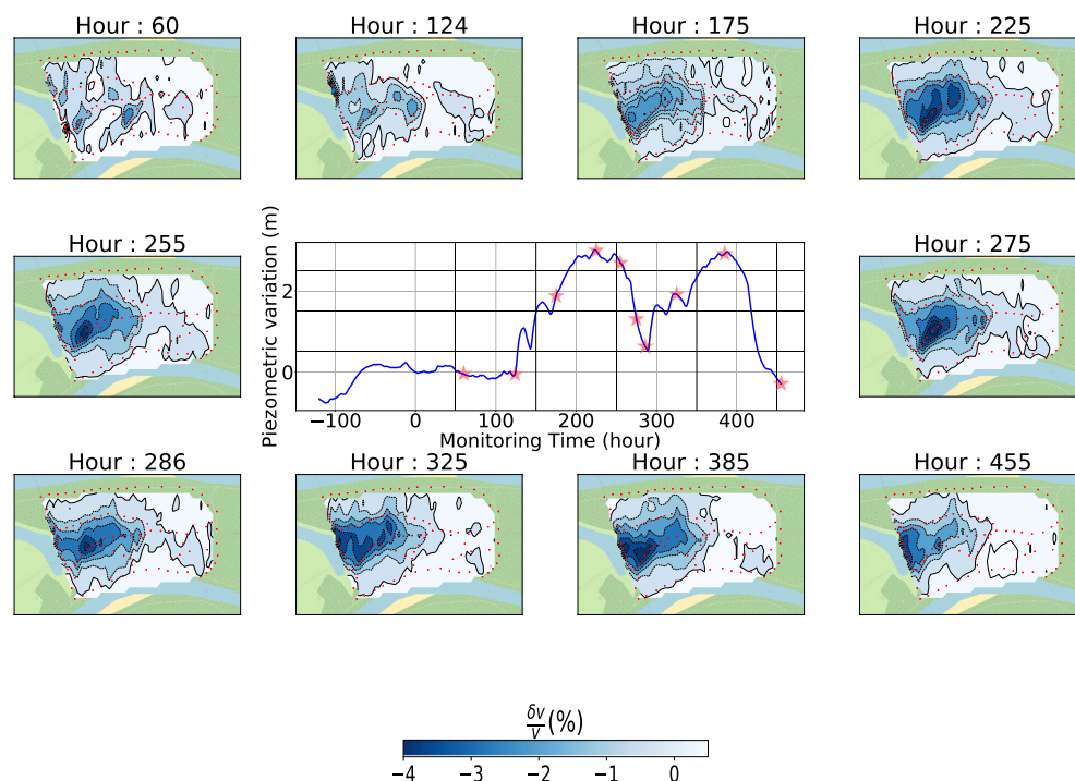
Figure 8. Evolution of the \delta v/v maps for 10 different key moments of the controlled monitoring experiments. The central graph shows the relative evolution of the water table measured at piezometer P95. The red stars highlight the moments for which the maps are shown.
