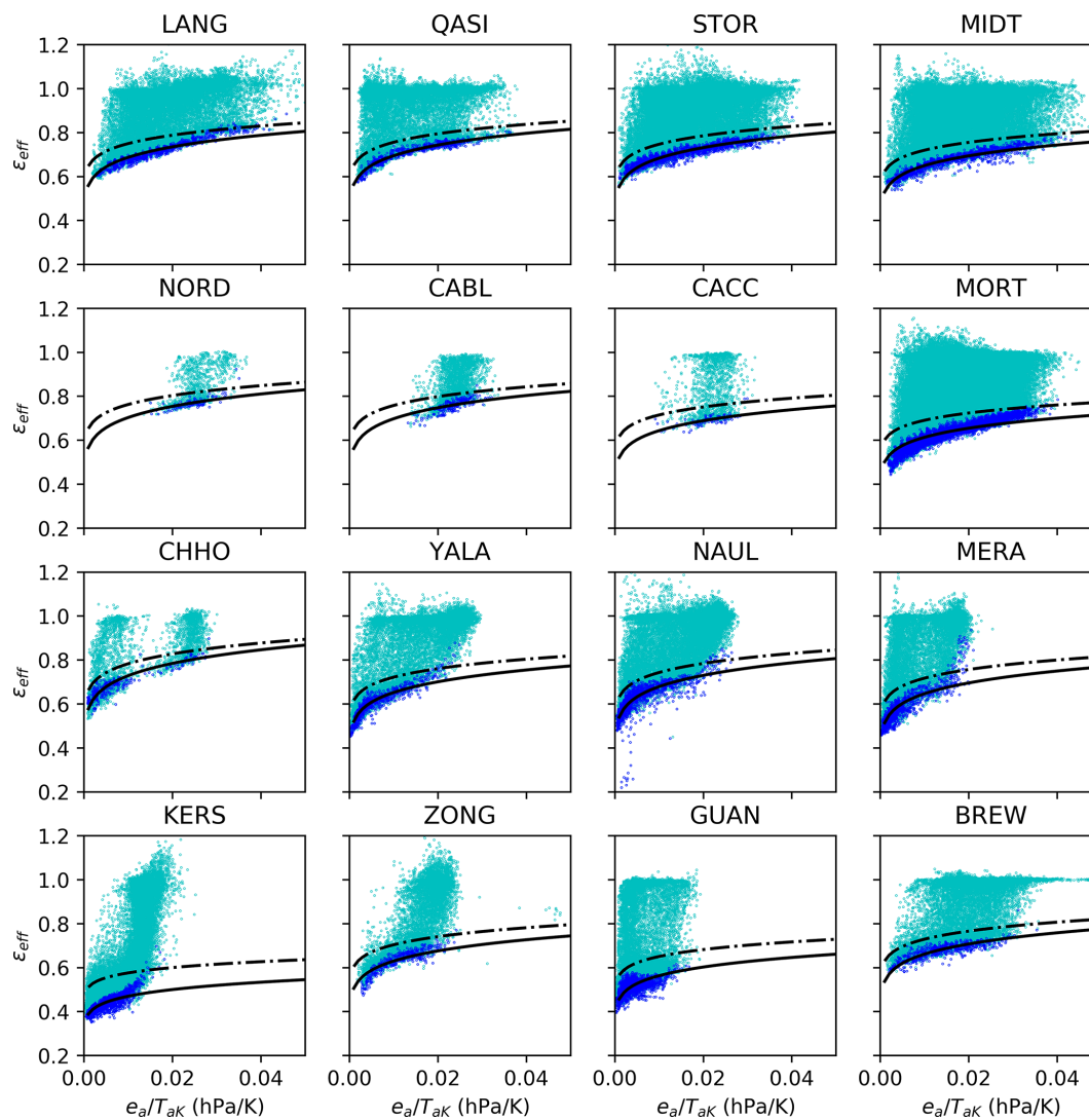
Figure A3. Observed \varepsilon_{\text{eff}} (points) and calculated \varepsilon_{\text{cs}} (solid line) fitted to lowest 10% of LWIn in 30e_a/T_{a,K} bins (shown in blue). Calculated \varepsilon_{\text{eff}} at clear-sky limit of N_\varepsilon = 0.2 (dash-dotted line).
