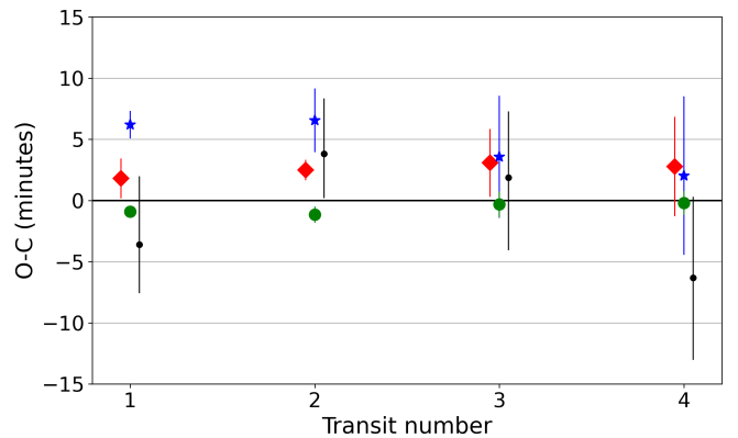
Fig. 10. Residuals for the mid-transit timings of TOI-1422 b versus a linear ephemeris, with 1-\sigma error bars, are plotted in black. The green circles, red diamonds, and blue stars represent TTV predictions in the cases of null, average, or maximum eccentricities, respectively, with the error bars showing the uncertainty due to T_{0,c} (see Table 2). The points have been slightly shifted on the x-axis to allow for more visibility.
