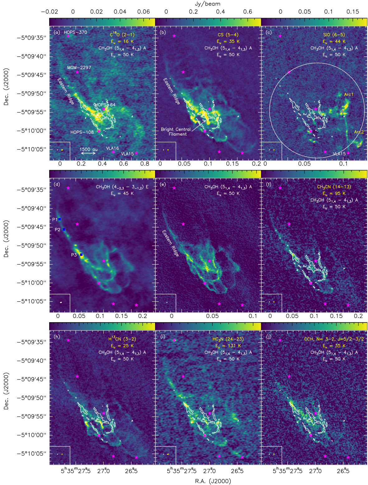
Fig. 1. Velocity-integrated maps of the different tracers used to probe the emission towards OMC-2 FIR 4. Upper panels: velocity-integrated maps of C^{18}O , CS and SiO in colours, with superimposed contours of the velocity-integrated emission of CH_3OH ( 5_{1,4}-4_{1,3} A ) line (white). The colour scale wedges are shown at the top of each panel. The different cores are depicted with magenta stars and are labelled in white. The synthesised beam of CH_3OH and the other molecules are depicted in the lower left corner in white and yellow, respectively. In the SiO panel, the positions of the SiO peaks from this study are depicted with filled grey triangles. The primary beam at the full width at half maximum is depicted in white. Middle panels: velocity-integrated maps of CH_3OH lines at E_u = 45 K and E_u = 50 K and of CH_3CN . On the latter, we superimposed the contours of the velocity-integrated emission of CH_3OH ( 5_{1,4}-4_{1,3} A ) line (white). The colour scale wedges are shown at the top of each panel. The positions of the three masers detected in CH_3OH ( 4_{-2,3}-3_{-1,2} E ) are depicted with filled blue squares. Lower panels: velocity-integrated maps of H^{13}CN , HC_3N and CCH in colours with superimposed contours of the velocity-integrated emission of CH_3OH ( 5_{1,4}-4_{1,3} A ) line (white). The colour scale wedges are shown at the top of each panel. The methanol contours start at 10\sigma with \sigma = 12.3 mJy beam ^{-1} km s ^{-1} .
