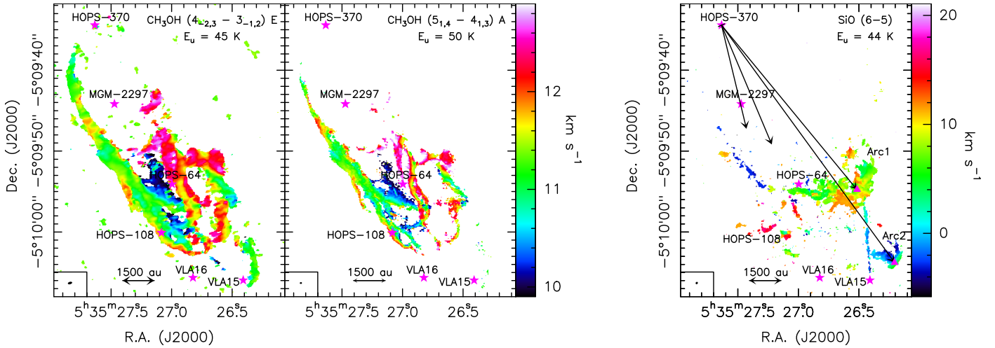
Fig. 3. Velocity maps of CH 3 OH and SiO towards OMC-2 FIR 4. Left panel: velocity maps (integrated between 9.9 and 12.9 km s -1 ; colour scale in km s -1 ) of CH 3 OH (4 -2,3 -3 -1,2 E) ( left ) and CH 3 OH (5 1,4 -4 1,3 A) ( right ). Right panel: velocity map (integrated between -6.2 and 24.4 km s -1 ; colour scale in km s -1 ) of SiO(6-5). The different cores are depicted with magenta stars and are labelled in black. The positions of the SiO peaks from this study are depicted with filled magenta triangles. We draw four arrows from HOPS-370, one perpendicular to the disk, two towards the SiO peaks, and one similar to the direction of the jet in [OI] by González-García et al. (2016) .
