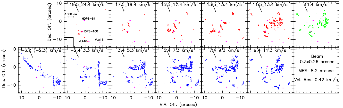
Fig. C.6. Channel maps of SiO. The contours are at [5, 20, 40]\sigma with \sigma = 2.5 mJy beam ^{-1} km s ^{-1} . The cores are depicted with magenta stars and are labelled in black. The synthesised beam is depicted in the lower left corner. We draw one arrow from HOPS-370 perpendicular to its disk. The beam, MRS, and velocity resolution values are reported in the bottom right panel.
