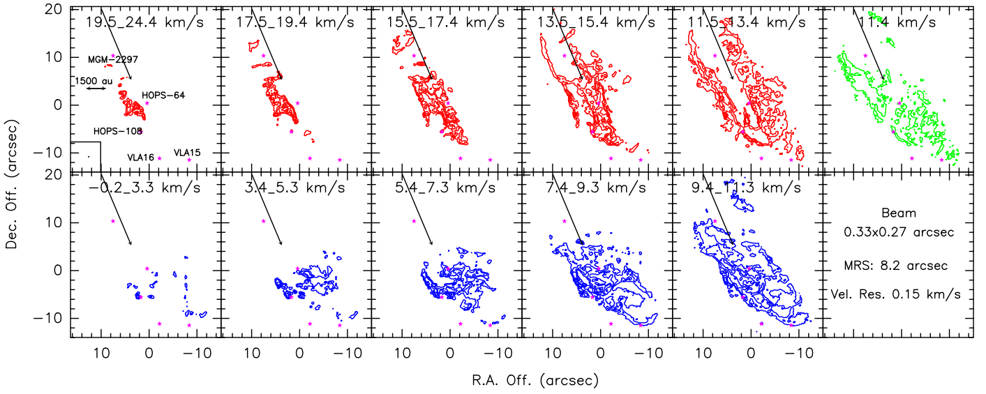
Fig. C.5. Channel maps of CS. The contours are at [5, 20, 40]\sigma with \sigma = 4 mJy beam ^{-1} km s ^{-1} . The cores are depicted with magenta stars and are labelled in black. The synthesised beam is depicted in the lower left corner. We draw one arrow from HOPS-370 perpendicular to its disk. The beam, MRS, and velocity resolution values are reported in the bottom right panel.
