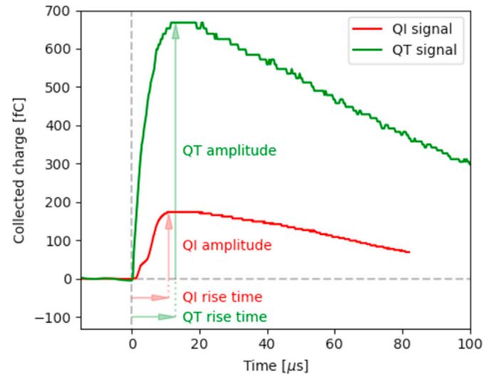
Fig. 10. QT and QI signals showing the negative and positive charges, respectively, which were collected at the detectors in the CDA over a few microseconds after a high velocity impact of a hollow silicate. A number of important measured properties - signal amplitudes and rise times - are schematically indicated by arrows.
