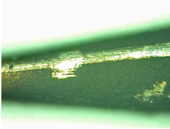
Fig. 3. The dust source needle, where carbon aerogel piled up and prevented further acceleration of carbon aerogel particles.
