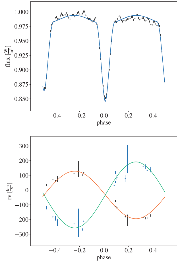
Figure 7. Top: Mean TESS light curve of WR 63 phase-folded with the 4.03 d period (black dots) and the fit (blue line) obtained from the orbital fitting using PHOEBE. Bottom: Radial velocity measurements and best-fitting RV curves of the O+O binary according to the solution listed in Table 2. The primary (secondary) is shown by black dots/orange line (blue dots/green line). Phase 0 corresponds to the primary eclipse.
