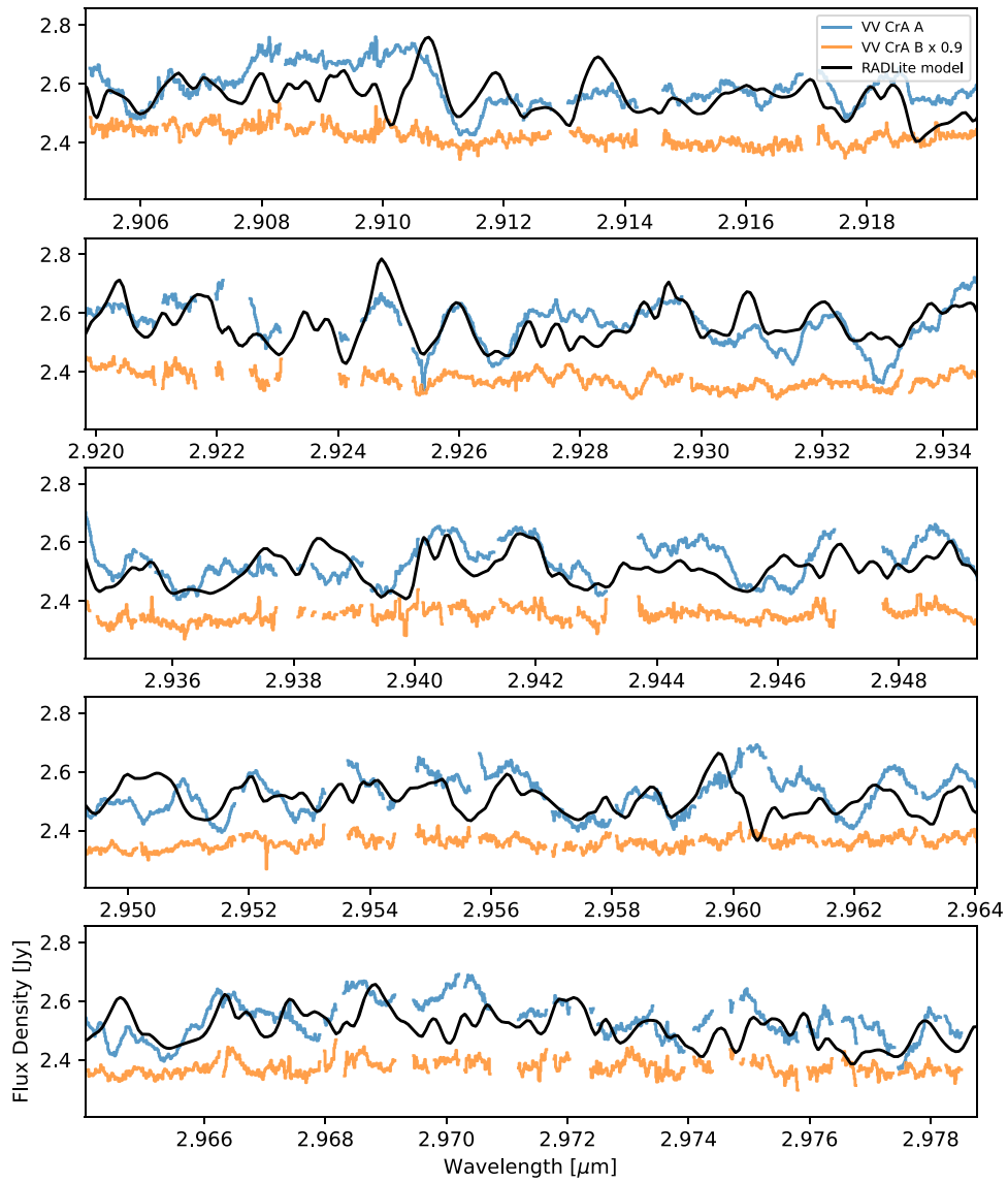
Figure A2. Reduced CRIRES spectra of VV CrA A and B in the L -band “H 2 O” setting.
