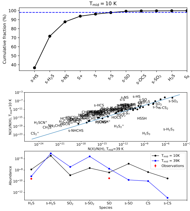
Fig. 11. Impact of varying the mid-plane temperature on the model results. Top : cumulative sulfur abundance fraction of the ten main sulfur carriers for the Nautilus model with T_{\text{mid}} = 10 K. Middle : abundance of sulfuretted species computed assuming T_{\text{mid}} = 10 K versus the abundance computed assuming T_{\text{mid}} = 39 K. We show the names of the species when there is an order of magnitude difference between both models, and plot black dots otherwise. Bottom : abundance of a subset of the most relevant sulfur carriers for the two mid-plane temperatures used.
