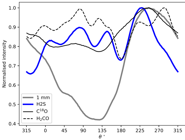
Fig. 4. H 2 S azimuthal cuts compared to previous observations by this team. All the intensity maps have been convolved to match the beam size of our H 2 S emission line maps. The azimuthal profiles shown were computed at the distance of the emission peak of each species. The profiles were normalized with respect to their respective peaks.
