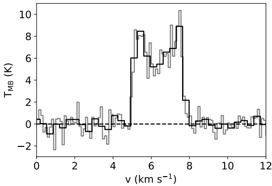
Fig. 2. Stacked H 2 S 1 01 –1 10 spectrum of AB Aur inside the 5 \sigma emission contour levels. The gray spectrum depicts the observed spectrum, and the black one depicts the same after rebinning.
