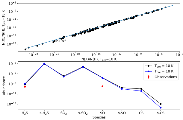
Fig. 12. Impact of varying the prephase temperature on the model results. Top : abundance of sulfuretted species computed assuming T_{\text{gas}} = 10 K versus the abundance computed assuming T_{\text{gas}} = 18 K for the molecular cloud prephase. Bottom : abundance of a subset of the most relevant sulfur carriers for the two prephase temperatures used.
