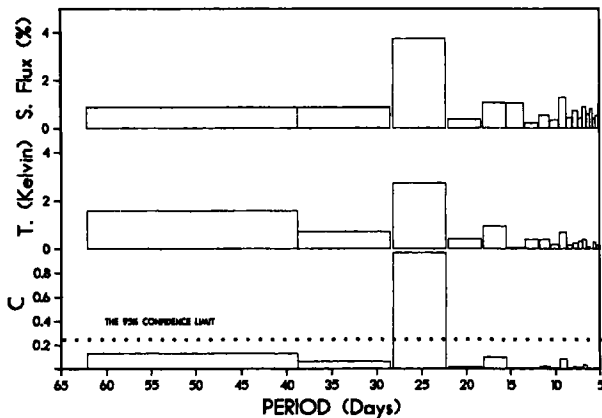
Fig. 2. Spectral analysis for the period between May to August 1985 : spectrum of the Lyman alpha solar flux (top), spectrum of the temperature at the altitude of 57 km (middle), and cross-spectrum between solar flux and temperature (bottom). Periods on the horizontal axis are expressed in days.
