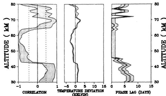
Fig. 6. As in fig 3 for the period between May to August 1985
