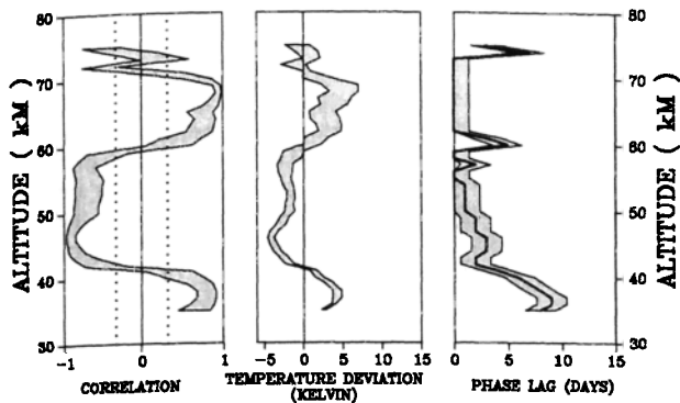
Fig. 4. As in fig 3 for the period between January to March 1983.
