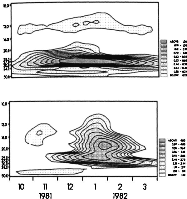
Fig. 5. Wavelet transform (as in fig 1) for the period from October 1981 to March 1982, of the solar flux (top) and the temperature at 55 km (bottom).
