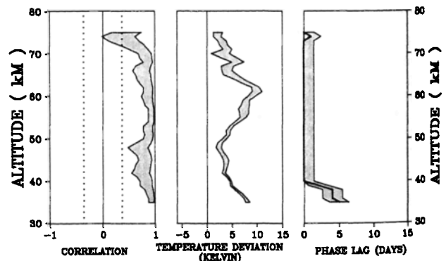
Fig. 3. Amplitude as a function of altitude of the 27-day spectral component for the period from January to March 1982. Correlation (left), temperature deviation (middle), and phase lag (right) between solar and temperature series are given. 95 % confidence level (dash line), phase lag uncertainties and white noise level (shaded area) are also plotted.
