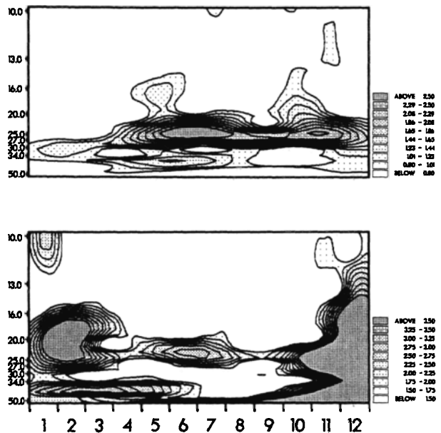
Fig. 7. As in fig 5 for the period from January to December 1985.
