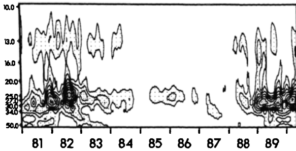
Fig. 1. Wavelet transform of the solar UV flux (Nimbus 7-NOAA 9) from 1981 to 1990. The horizontal axis represents the time (in years) vertical one the periods (in days).
