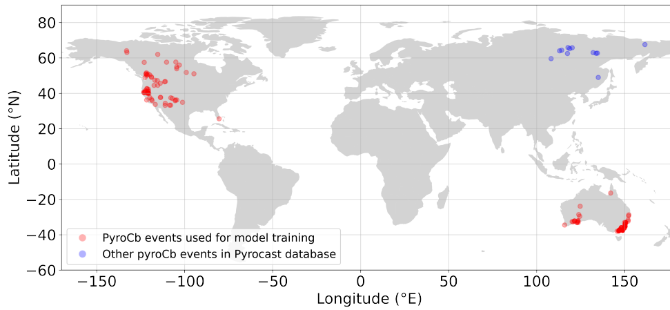
Figure 6: Spatial distribution of pyroCb events in the PYROCAST database.
