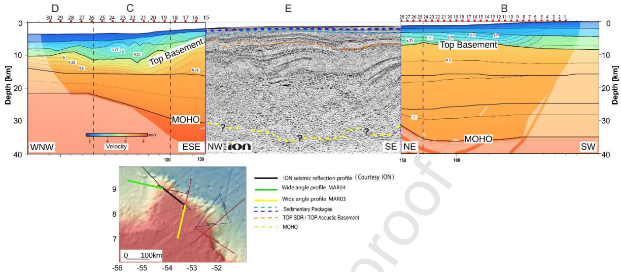
Figure 13: Composite depth image of the seismic velocity models derived from wide angle seismic profiles MAR 04 and MAR 03 combined at the intersection with the connecting depth migrated multi-channel seismic reflection profile (Seismic reflection data courtesy of ION). Inset map shows location of the three profiles
