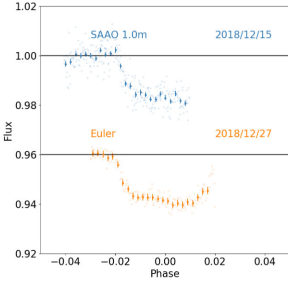
(a) Additional Photometry for NGTS-23b.
