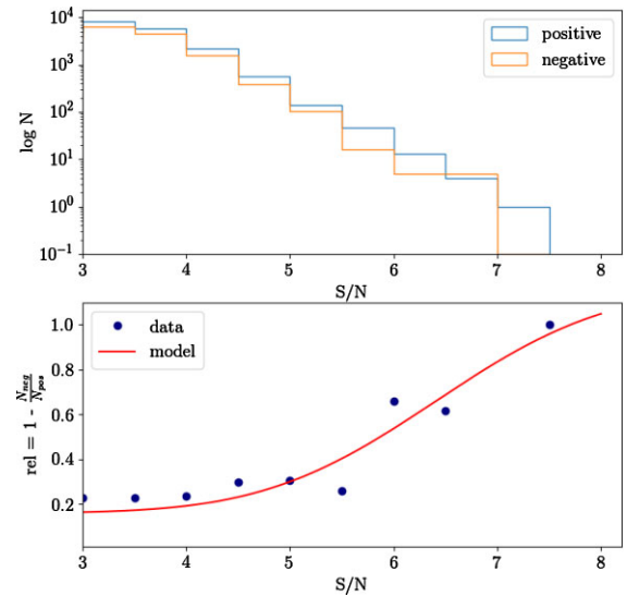
Figure 8. Calculating the reliability coefficient. The top panel shows the distributions of peak signal-to-noise ratio for the positive and negative detections. The surplus of positive detections defines the reliability coefficient. The bottom panel shows the reliability model (equation 2) fitted to the ratio of negative versus positive detections (equation 1). Thanks to the model, we can calculate the reliability coefficient at any signal-to-noise ratio.
