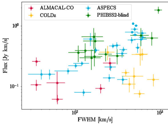
Figure 6. The integrated flux and width of the CO candidates from ALMACAL-CO (red) compared to detections from other untargeted surveys: ASPECS (blue, Decarli et al. 2019), COLDz (yellow, Riechers et al. 2019), PHIBSS2 (green, Lenkić et al. 2020). ALMACAL-CO detections are fainter and narrower compared to the detections from other surveys.
