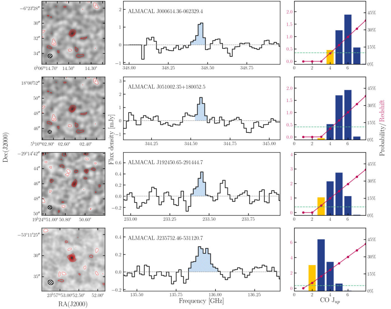
Figure 5. ALMACAL-CO emission lines candidates. Left-hand panel: ALMA 0th-moment map centred on the detection candidates discovered in the ALMACAL-CO untargeted search. The contours correspond to \pm 3\sigma , 4\sigma , 5\sigma , 6\sigma , derived from the respective line map. The size of the synthesized beam is shown in the lower left-hand corner. The grey areas mark the parts of the primary beam that were not included in our image cut. Middle panel: spectrum of the line candidates at the brightest pixel. The blue dashed region marks the spectral extent of the detected line. Right-hand panel: The distribution of CO transitions predicted by SHARK corresponding to ALMACAL-CO line detections. The majority of sources in our sample are associated with J_{\text{up}} = 4, 5, 6 . The parameters of all candidates as summarized in Table 2. The lowest possible J_{\text{up}} is marked in yellow. The red line indicates the redshift (left y-axis) of the corresponding J -transition in the histogram. The green horizontal dashed line marks the redshift of the calibrator in that field, indicating that the emitters do not preferentially cluster around the calibrator. For the candidates from field J0334-4008 (Fig. 4), we choose the CO(1 – 0) solution with probability 100 per cent, as confirmed by the optical counterparts.
