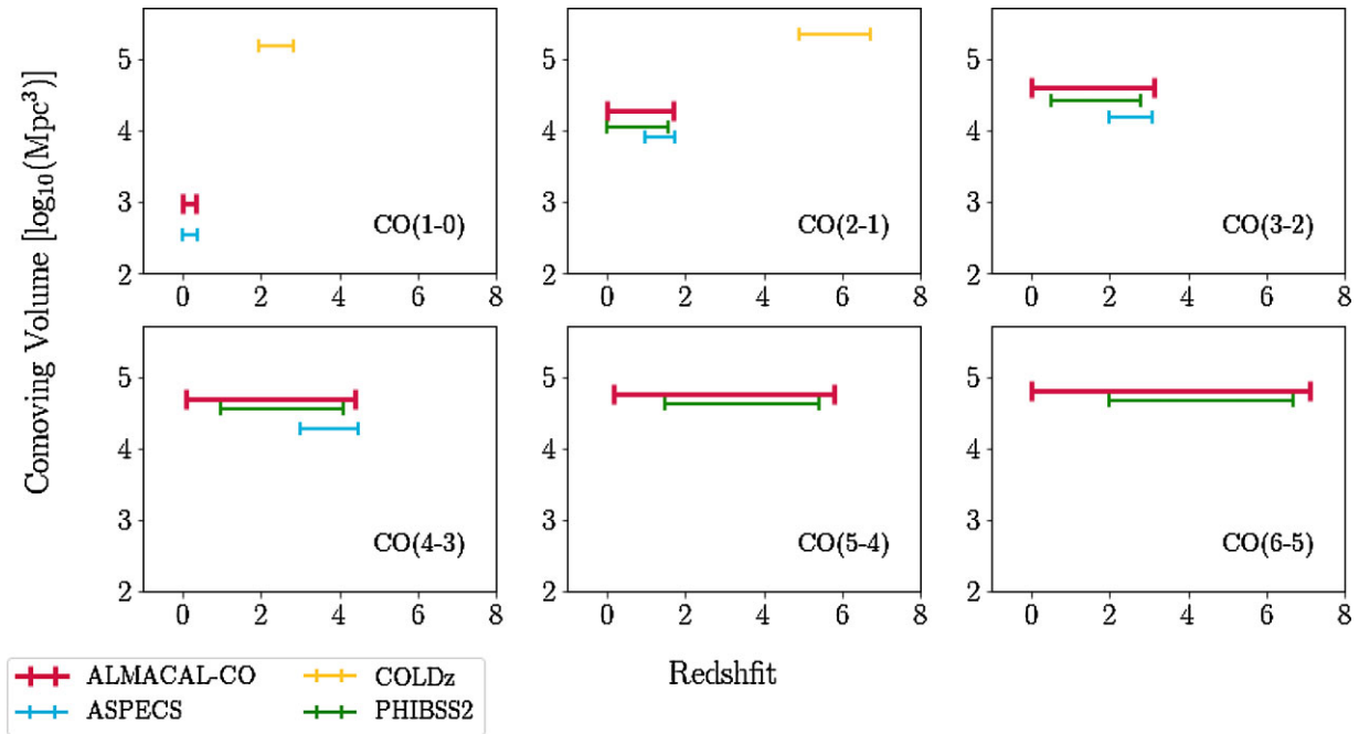
Figure 10. Comparison of volume coverage for CO transitions from J_{\text{up}} = 1 - 6 in ALMACAL-CO pilot (red), ASPECS – blue Decarli et al. 2019, PHIBSS2 – green, Lenkić et al. 2020 and COLDz – yellow Riechers et al. 2019). ALMACAL-CO pilot covers a larger volume for individual transitions (except for high redshift COLDz) thanks to the large frequency span.
