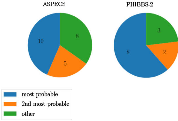
Figure A1. Number of correctly identified transitions of the sources from ASPECS (left-hand panel, Decarli et al. 2019) and PHIBSS2 (right-hand panel, Lenkić et al. 2020) surveys by our SHARK-based redshift calculator. The blue slice depicts the number of transitions for which the identification as most probable is consistent with the spectral classification. The orange slice covers transitions for which the most probable J_{\text{CO}} was one lower/higher than the classified one (and the actually observed transition was assigned significant probability), while the green slice covers all other cases. The redshift calculator identifies correctly about 50 percent of the detections (over 60 per cent if we include the ‘second most probable’ option).
