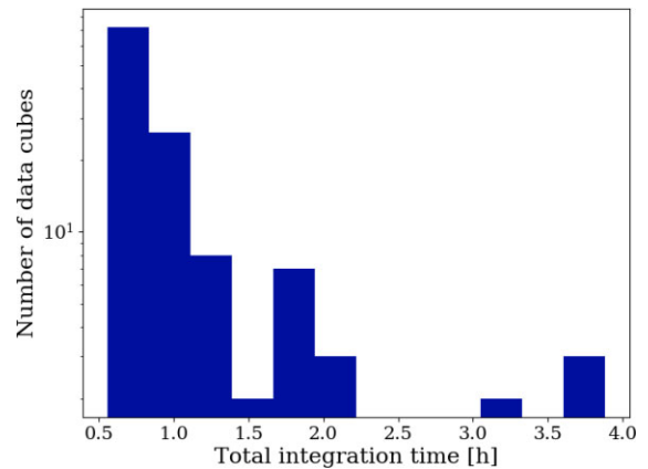
Figure 2. Total integration time distribution of the ALMA data cubes used in this study. The lowest integration time is limited to 40 min by construction. The longest integration time typically reaches 2 h with a few exceptions of even longer observations. The total integrated time results from concatenating the short (several minutes) singular calibration pointing taken in the same spectral setup.
