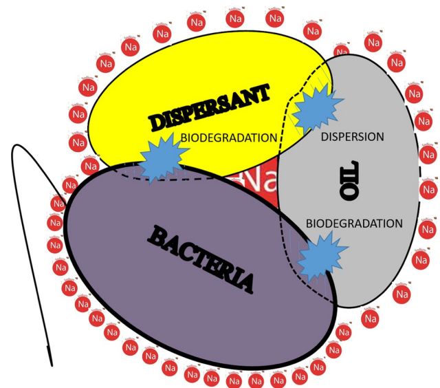
Fig. 3 Role of bacteria in oil/dispersant biodegradation under saline water conditions
