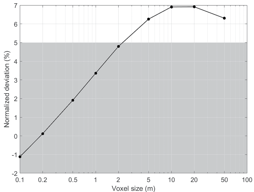
Figure 12. The normalized FAPAR deviation of voxel-based RT simulation under different voxel sizes. Results of the 3D-explicit RT simulation with the same simulation settings were used as the benchmark. The gray area indicates the 5% tolerance region.
