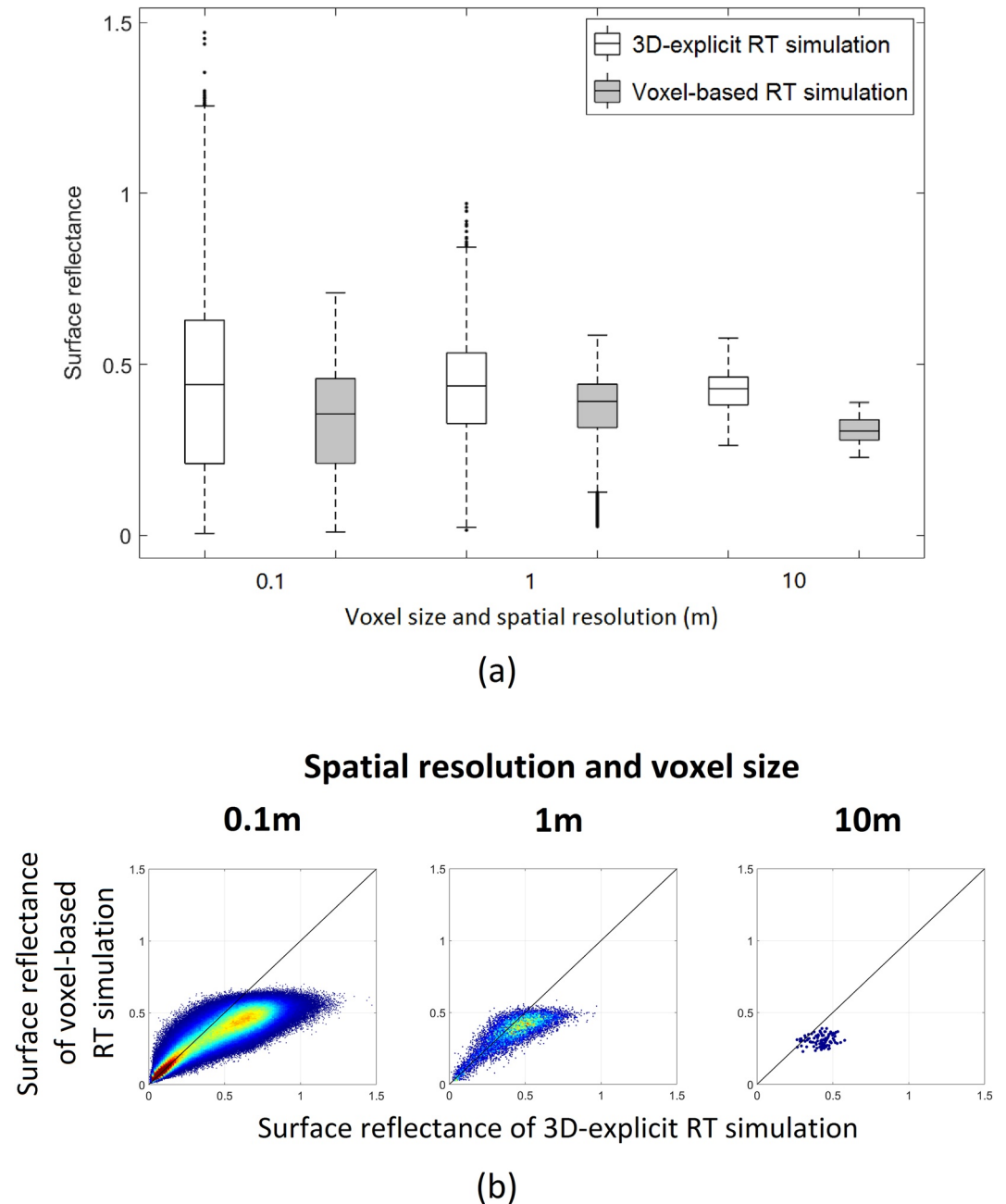
Figure A4. Statistics of pixel surface reflectance (ps) values of nadir NIR images. (a) Boxplot of surface reflectance of each image. Gray boxes are statistics of images of voxel-based RT simulations, under the same simulation conditions as the 3D-explicit images on their left. (b) Scatter plots that compare the surface reflectance of different RT simulations pixel by pixel, in spatial resolutions and voxel sizes 0.1 m (left), 1 m (middle), and 10 m (right). The solid black line represents the 1:1 line.
