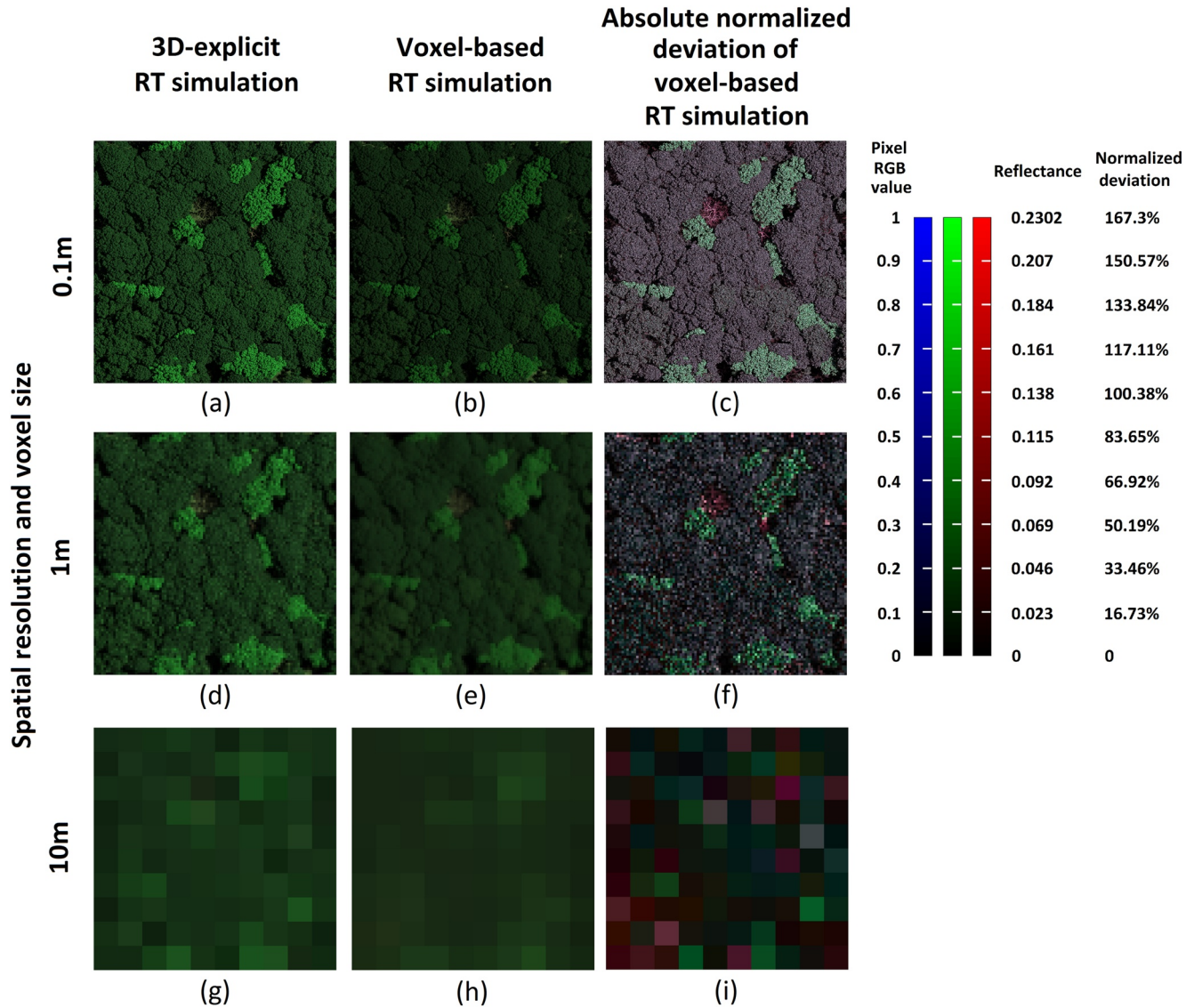
Figure 5. Simulated nadir surface reflectance ( \rho_s ) images and deviation images over the 1-ha Wytham Woods plot, with spatial resolutions and voxel sizes 0.1 m (first row), 1 m (second row), and 10 m (third row), respectively. First column: RGB surface reflectance images of 3D-explicit RT simulation. Second column: RGB surface reflectance images of voxel-based RT simulation. Third column: RGB images of absolute normalized deviation of voxel-based RT simulation; results of the 3D-explicit RT simulation with the same simulation settings were used as the benchmark, and the absolute values of normalized surface reflectance deviation in red, green, and blue wavebands were transformed into pixel RGB values. The correspondence between pixel RGB values and reflectance/deviation values is: pixel R, G, and B values 0–1 correspond to reflectance 0–0.2302, and normalized deviation 0 to +167.3%. The images are based on bands 2, 3, and 4 from the MSI instrument on Sentinel-2 (wavelength: 490 \pm 32.5 , 560 \pm 17.5 , and 665 \pm 15 nm). The simulated sensor was placed at the Bottom of Atmosphere (BOA). For the images of voxel-based RT simulation, the spatial resolutions are equal to the voxel size.
