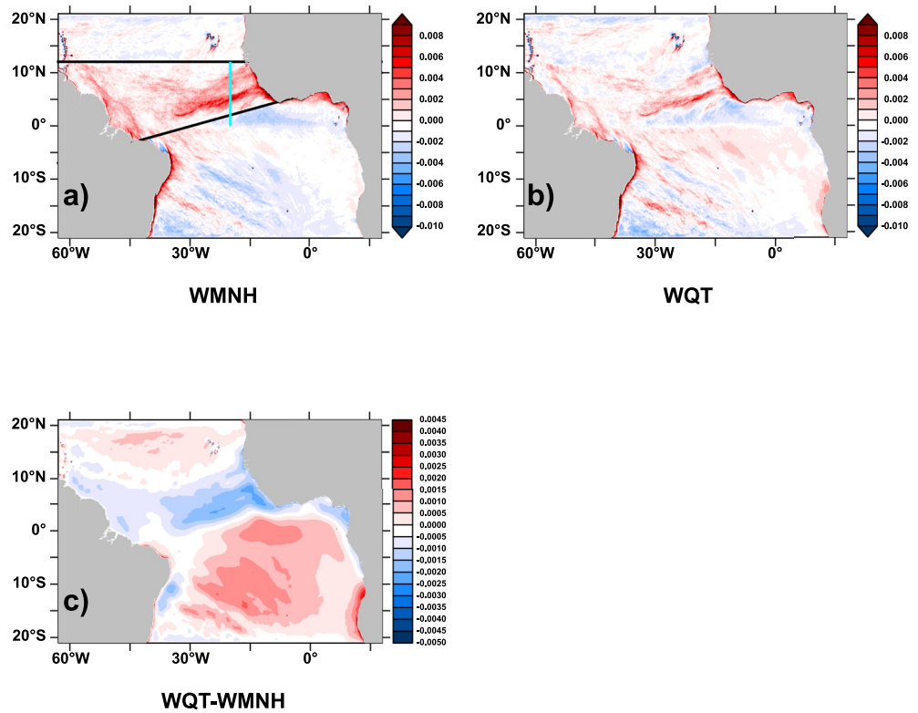
Figure 7. June averaged boundary-layer (a) simulated vertical velocity ( WMNH , m s^{-1} ). The black lines bound the AMI region which correspond to maxima of vertical velocity. The blue segment is the track of the vertical Section across the AMI where occur the most intense ascending motions. (b) Retrieved vertical velocity ( WQT , m s^{-1} ) after inversion of \omega -Equation 2 and (c) difference WQT - WMNH ( m s^{-1} ).
