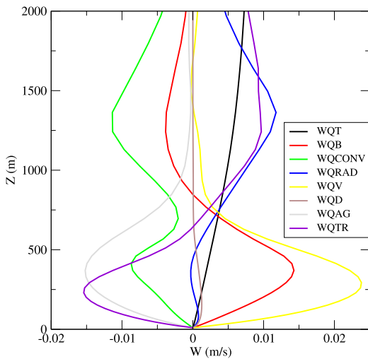
Figure 18. Vertical distributions of vertical velocity components ( \text{m s}^{-1} ) averaged over the AMI domain (see Figure 7).
