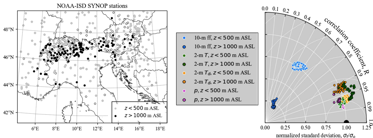
Fig. 3. Verification of hourly forecasts of 2-m temperature (2-m T ), dewpoint (2-m T_d ), 10-m wind speed (10-m ff ), and surface pressure ( p ) by the ECWMF IFS model (1200 UTC run) in the period 2016–19, for forecast ranges between 0 and 48 h. (left) Synoptic stations in and around the Alps, available in the NOAA Integrated Surface Database downloaded from the Global Hourly-Integrated Surface Database of NOAA ( www.ncei.noaa.gov/products/land-based-station/integrated-surface-database , accessed on 4 Nov 2021; Smith et al. 2011). Black: station height > 1000 m MSL (proxy for mountain site), gray: station height < 500 m MSL (proxy for flat terrain site). (right) Taylor diagram contrasting mountain and flat terrain sites (as depicted in the left panel) for different variables (coloring: see inset). Each point in the Taylor diagram refers to a specific forecast range and represents a spatially averaged score, i.e., the mean value across all observing sites in the set. Variability around the mean is large, especially in the case of wind speed forecasts (not shown). The Taylor diagram relates the correlation coefficient between observed and modeled values ( R ) to the respective standard deviations ( \sigma_f for the standard deviation of the forecast, \sigma_o for the standard deviation of the observations). Perfect forecasts and forecasts affected by a constant bias would have R = 1 and \sigma_f/\sigma_o = 1 (black half-dot on the horizontal axis); distance from this point is proportional to the root-mean-square error of debiased forecasts. For the model output of the deterministic IFS forecast, see data availability statement.
