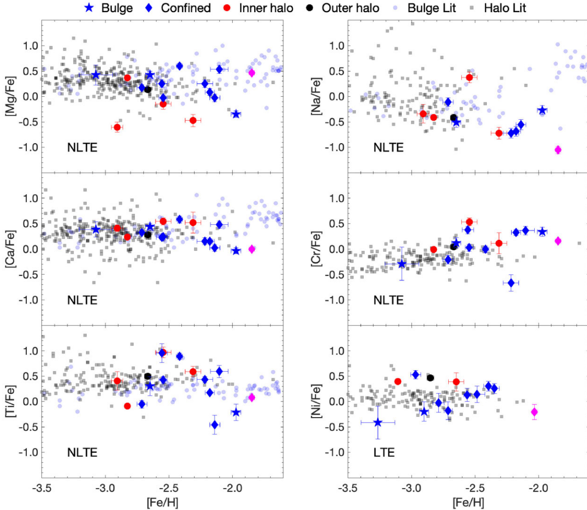
Figure 8. Chemical abundances ratios as a function of [\text{Fe}/\text{H}] . \alpha – elements Mg, Ca, and Ti are displayed on the left-hand panels, Odd-Z Na is on the top right, and the Fe-peak elements Cr and Ni are on the central and bottom right panels. All the panels, except [\text{Ni}/\text{Fe}] versus [\text{Fe}/\text{H}] , are corrected by NLTE effect as discussed in Section 6.6. The stars in the PIGS/GRACES sample are marked with the same symbols and colours as Fig. 4. The bulge literature sample (blue circles) is composed by stars from Howes et al. (2014, 2015, 2016), Koch et al. (2016), Reggiani et al. (2020), and Lucey et al. (2022). Halo literature compilation (grey squares) are from Aoki et al. (2013), Yong et al. (2013), and Kieley et al. (2021).
