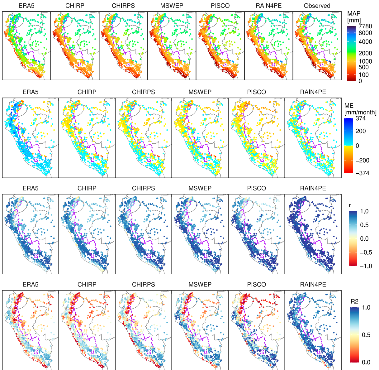
FIG. 6. Performance of the unadjusted precipitation datasets in comparison with gauge observations: MAP is the mean annual precipitation, ME is the mean error, r is the Pearson's correlation coefficient, and R^2 is the coefficient of determination. The comparison measures (ME, r , and R^2 ) were computed using monthly precipitation time series for 1981–2015.
