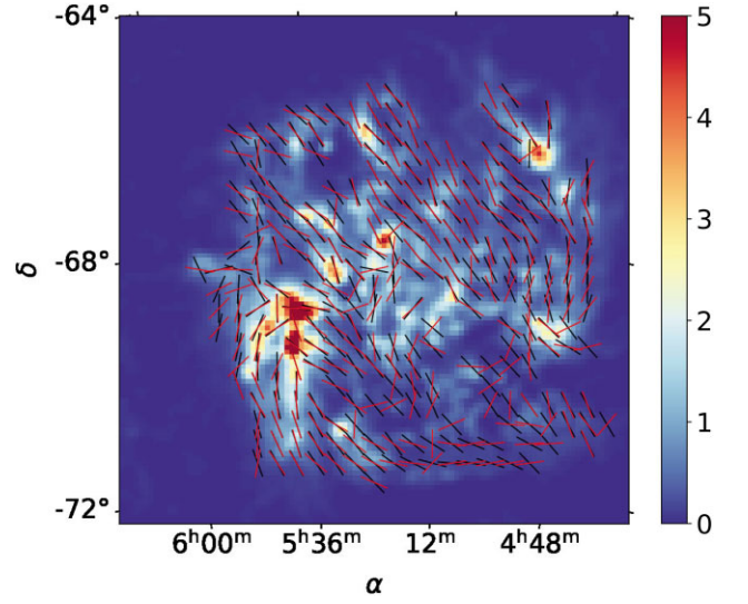
Figure A2. Map of the LMC 353 GHz intensity after foreground removal overlaid with segments showing the direction of the magnetic field derived from the Planck data at 335 GHz. The black and red segments show the geometry of the field before and after foreground removal, respectively. The directions are not shown for pixels outside the mask defined in Section 4.
