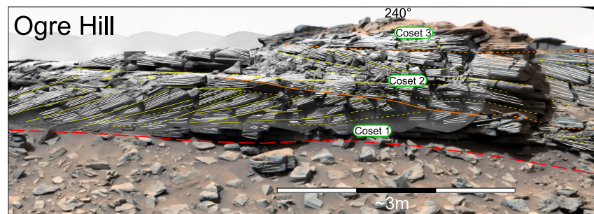
Figure 11. OGRE Hill composite mosaic. Apparent dip-azimuth of coset one is toward the south, which suggests that the lower Gleann Beag interval is absent from this outcrop. Overlying coset 2, and 3 record reversals of dip azimuth, suggesting further flow reversals. Interpreted high-resolution image of Figure 11. (Composite image: MR_mcam14367, acquired on Sol 2741, with ChemCam RMI CCAM04740, at Sol 2734 end-of-drive location). Image credit: NASA/JPL-Caltech.
