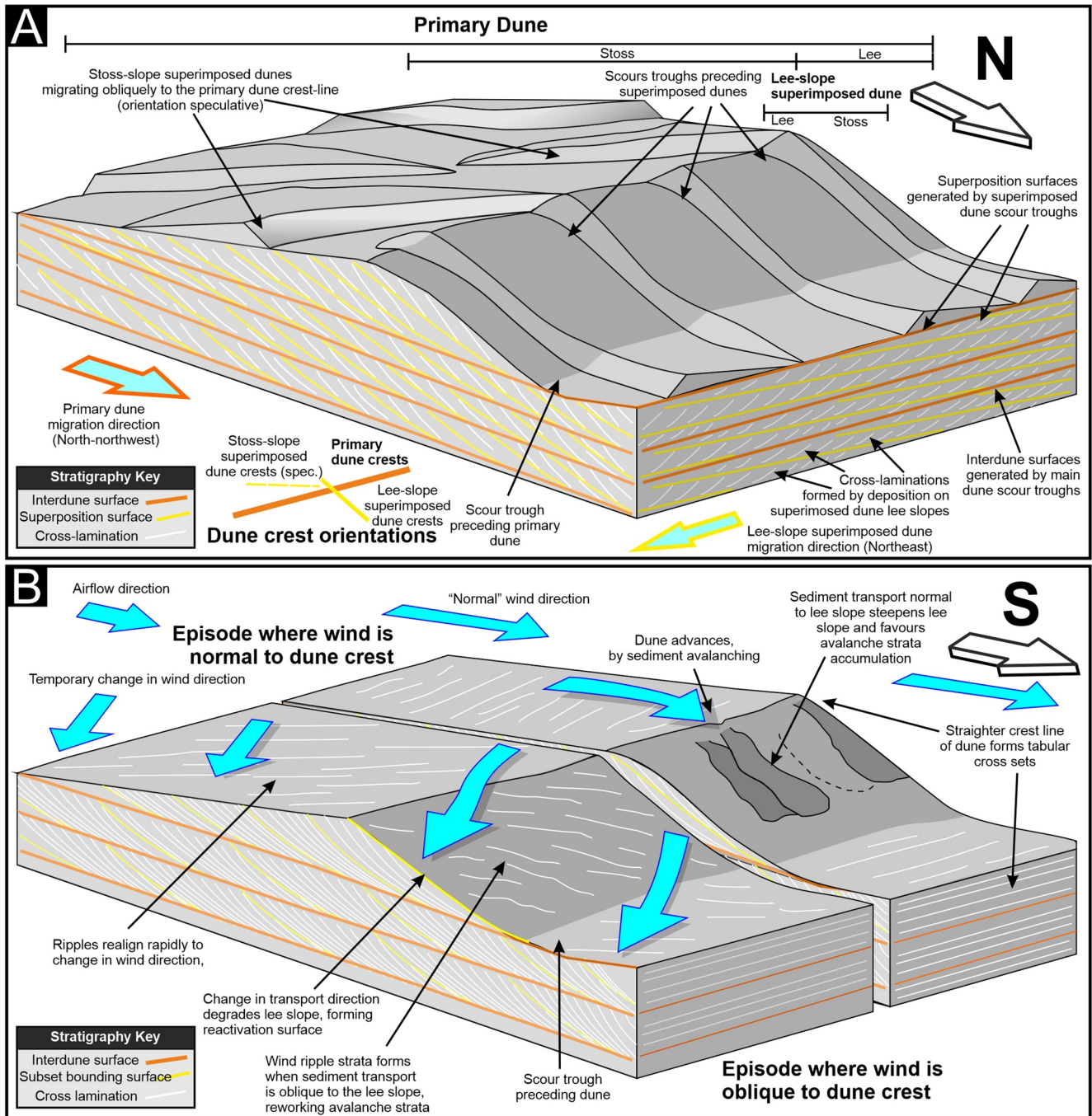
Figure 13. Reconstruction of bedforms interpreted from the Stimson formation exposed the Greenhugh pediment. (a) Schematic representation of compound bedforms interpreted to have deposited the Gleann Beag section. Primary dune lee-slopes are interpreted to dip toward the north or north-north west. Lee-slope superimposed dunes are interpreted to be migrating roughly toward the northeast, while stoss-slope superimposed dunes inferred (see text for details). (b) Schematic representation of bedform responsible for depositing the Ladder section.
