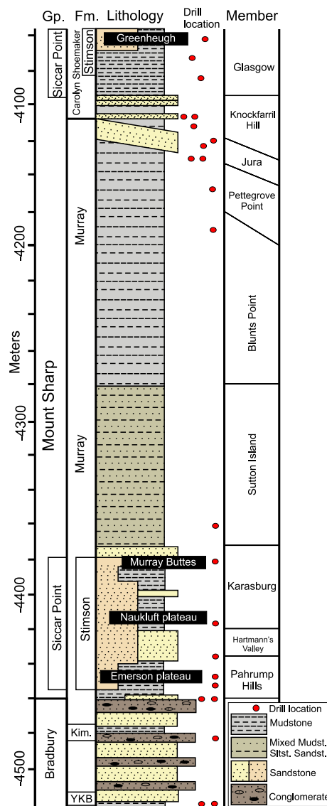
Figure 2. Stratigraphic context of the Simson formation within the stratigraphic framework erected by the MSL team. The stratigraphic column depicts key stratigraphic units encountered by the rover during the mission. The column shows units associated with the vertical elevation and does not account for total stratigraphic thickness. Members referred to form components of the Murray and Carolyn Shoemaker formations. For more details see Fedo et al., 2022; Caravaca et al., 2022; Bennett et al., 2022.
