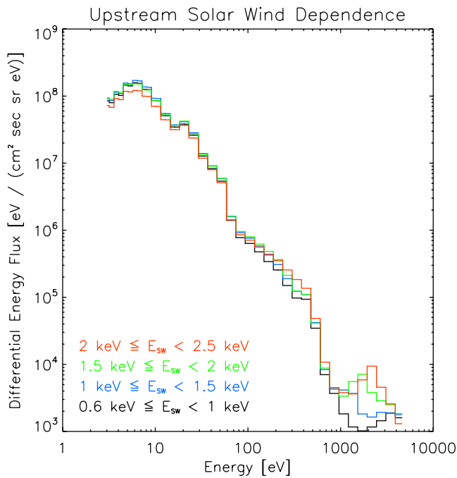
Figure 4. Four flux–energy spectra, averaged over solar wind energies. The spectra were calculated using the background–corrected anti–sunward spectra of the individual orbits. H^- ions were detected above \sim 800 eV for solar wind energies above 1 keV. At higher solar wind energies, both the peak flux and the peak energy of the H^- ions increase.
