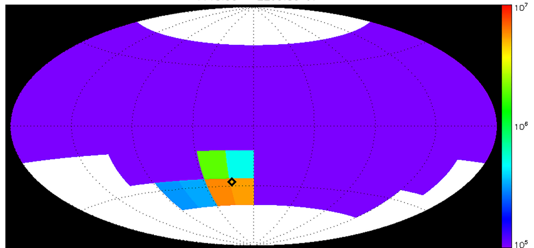
Figure 2. Angular distribution of high-energy (2–4 keV) Solar Wind Electron Analyzer differential energy flux ( \text{eV}/\text{cm}^2 \text{ sec sr eV} ) measured at low altitude. The black diamond indicates the sunward-looking direction (i.e., anti-sunward particle velocities). The space angle is 4\pi , and counts are collected over the full mass/charge range.
