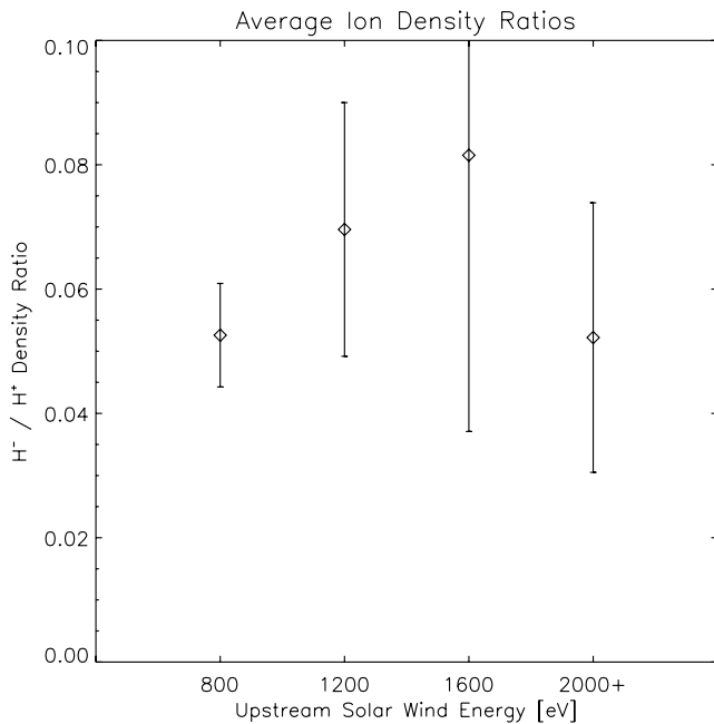
Figure 7. Average H - /H + density ratios for four solar wind energy bins, each 400 eV wide. H - densities were calculated using Solar Wind Electron Analyzer differential energy fluxes, and H + densities were calculated using Solar Wind Ion Analyzer penetrating proton measurements. Error bars correspond to the standard error of the mean.
