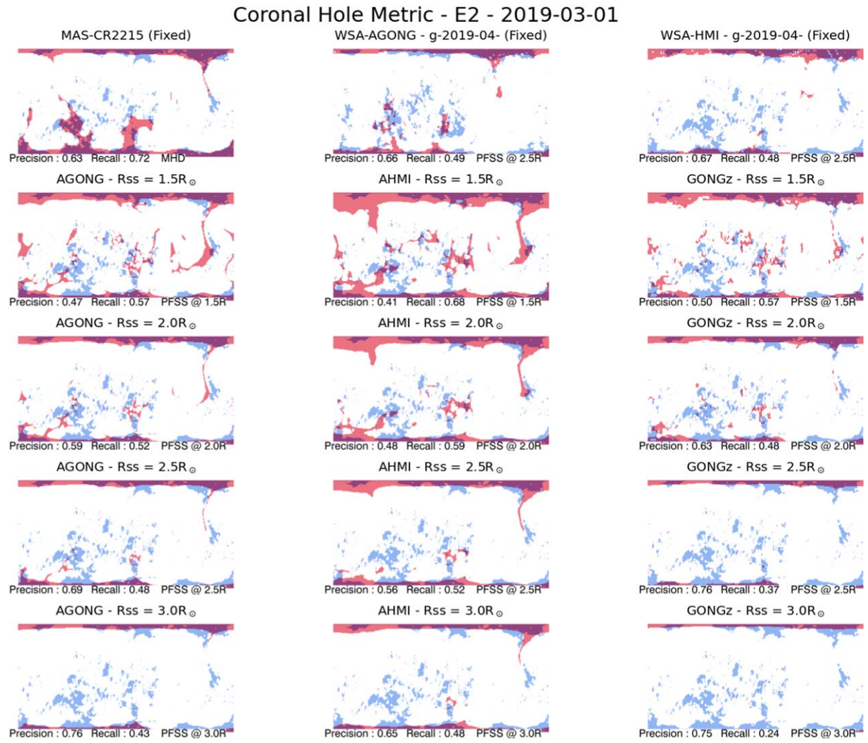
Figure 9. Metric 1 (Coronal Hole) model-observation comparison for the second PSP encounter. The panels are organized as in Figure 8. The online animation shows daily evolution from 2019 March 1 to 2019 April 30 except for the MAS and WSA models (top row), which are based on a single magnetogram for this encounter. (An animation of this figure is available.)
