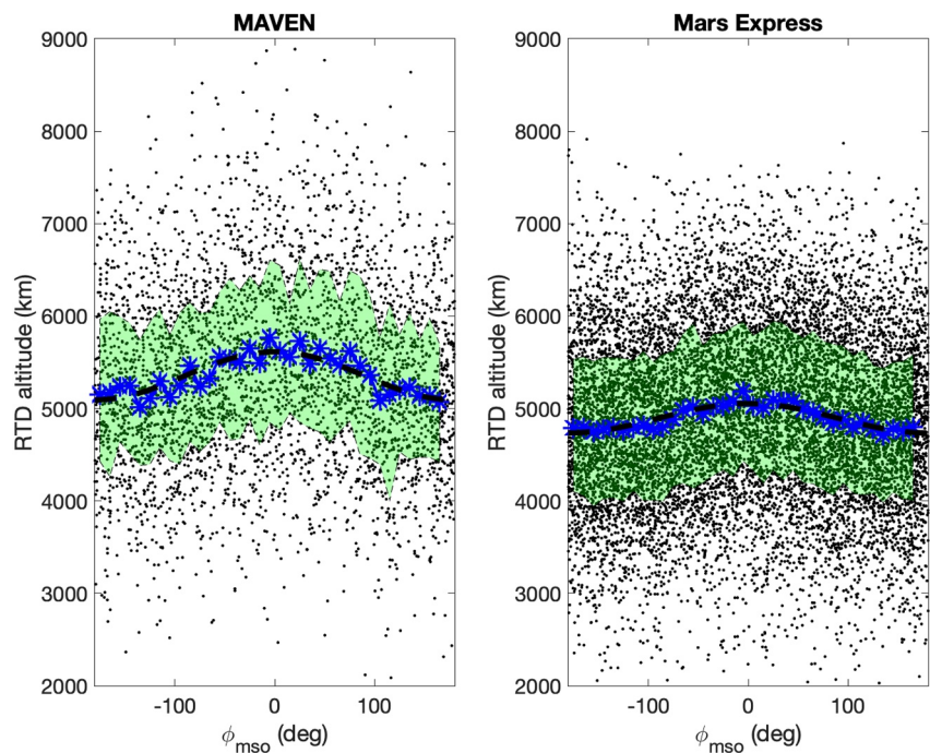
Figure 4. Mars Atmosphere and Volatile Evolution (left) and Mars Express (right) shock R_{TD} terminator altitude as a function of \phi_{mso} the MSO longitude of the strongest crustal source region center: 0^\circ at noon, +90^\circ at dusk -90^\circ at dawn. The mean observed profile (blue stars) is compared with a simple cosine fitting (black dashed line). The shaded area covers the 20%–80% percentiles range of shock terminator altitudes.
