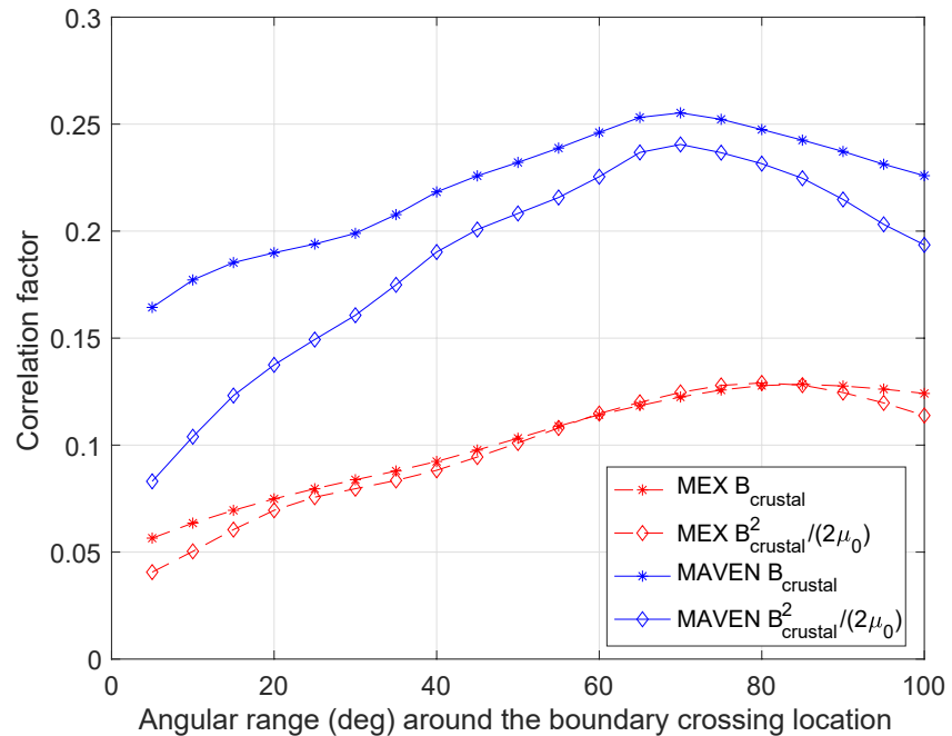
Figure 2. Correlation factor between the R_{TD} terminator altitude of the shock crossings (for Mars Atmosphere and Volatile Evolution in blue, for Mars Express in red) and crustal magnetic field pressure or intensity. The crustal field magnetic field intensity or pressure are taken from the Morschhauser et al. (2014) model at 400 km altitude at the sub-spacecraft position (same IAU longitude and latitude) below the crossing, then averaged over an angular range around the sub-spacecraft location. The correlation factor is given as a function this angular range, to reveal whether the crustal field influence on the shock location is local or global.
