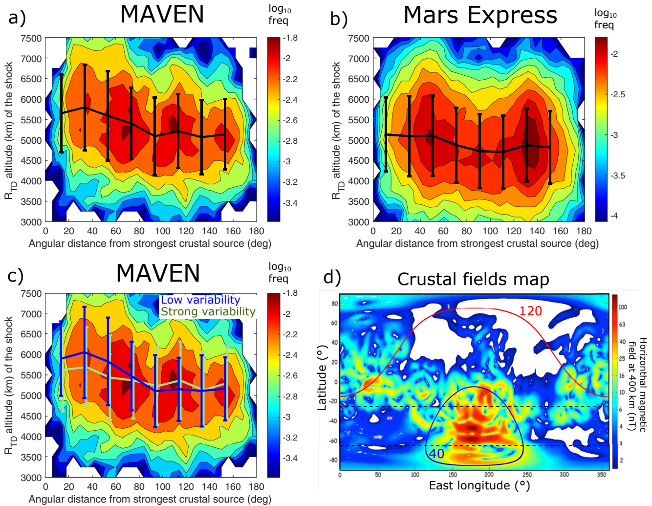
Figure 3. Logarithmic occurrence frequency of the shock crossings distributions for the Mars Atmosphere and Volatile Evolution (panel a and c) and Mars Express (panel b) datasets as a function of the terminator altitude and of the angular distance from the strongest crustal source region center (see text for details). The mean and standard deviation are superimposed. Panel (c) same distribution as panel a, with means and standard deviations for either low or strong IMF clock angle orientation variabilities preceding the BS crossings. Panel (d) geographical map of the horizontal crustal magnetic field at 400 km altitude, with isocontours of the angular distance from the strongest crustal source region (blue line for 40°, red line for 120°) and two isolatitude lines at -25^\circ and -65^\circ .
