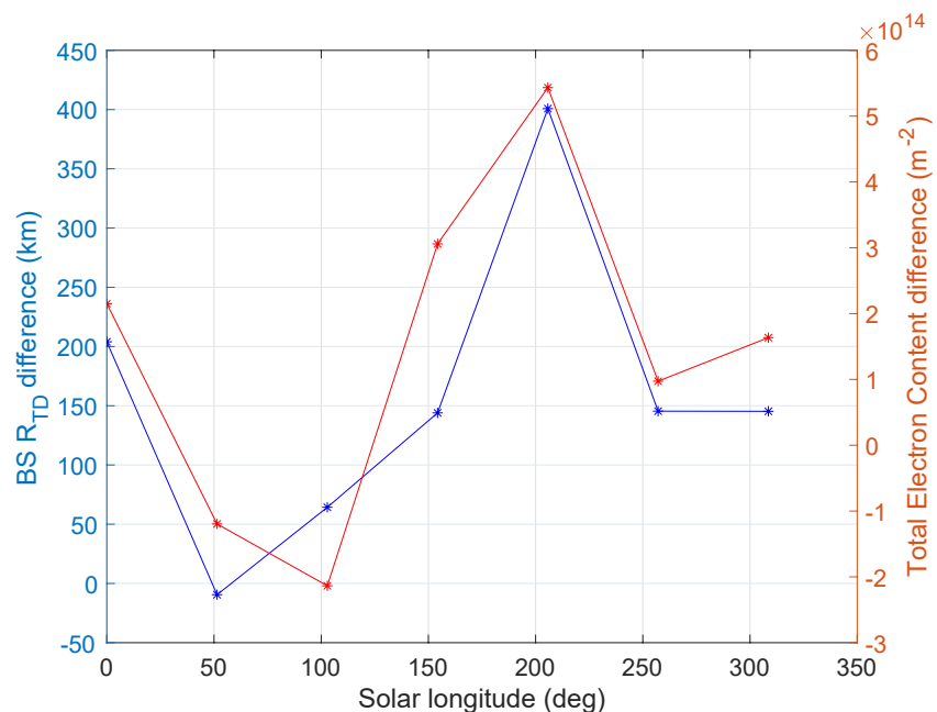
Figure 6. Compared seasonal variation of both the Total Electronic Content (TEC) of Mars ionosphere given by Mars Express (MEX) MARSIS data, and of the MEX bow shock R_{TD} extrapolated terminator altitudes. For both parameters at each season, we show the difference between the value close versus away the strongest crustal field source region (when only focusing on the southern hemisphere \pm 20^\circ latitude band considered in Figure 1; see text for more details). The solar longitude (Ls) of Mars is the Mars-Sun angle measured from the Northern Hemisphere spring equinox where Ls = 0^\circ ( Ls = 90^\circ corresponds to northern summer solstice, Ls = 180^\circ to northern autumn equinox).
