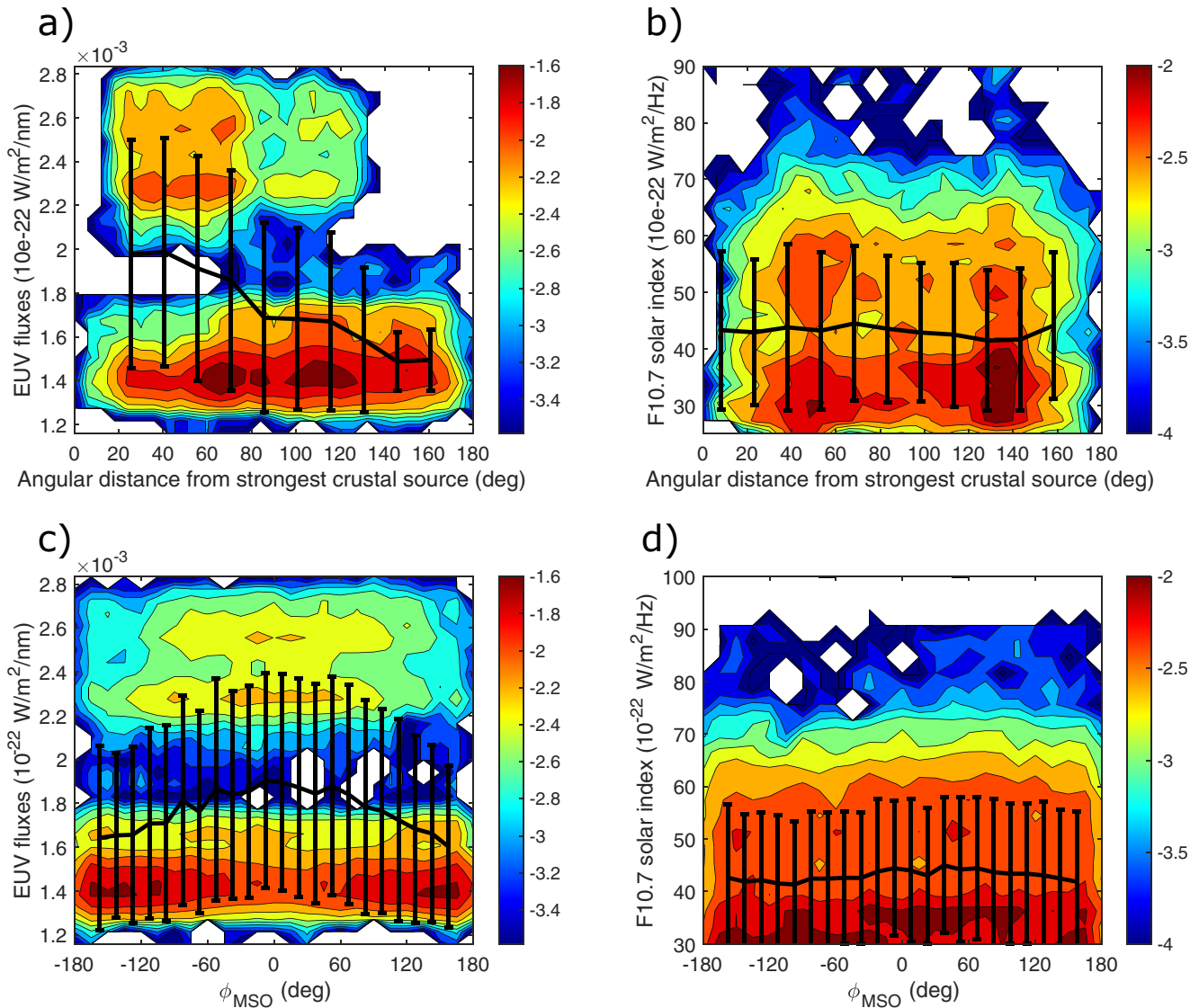
Figure 5. Logarithmic occurrence frequency of the shock crossings distributions for the Mars Atmosphere and Volatile Evolution (MAVEN) (left panels a and c) and Mars Express (right panels b and d) datasets as a function of the extreme ultraviolet fluxes (given by the FISM extreme ultraviolet fluxes for MAVEN and by the solar 10.7 cm radio flux index extrapolated to Mars for Mars Express) and of 1) either the angular distance from the strongest crustal source region (upper panels a and b) 2) or \phi_{\text{MSO}} the MSO longitude of the strongest crustal source region (lower panels c and d). The mean and standard deviation are superimposed.
