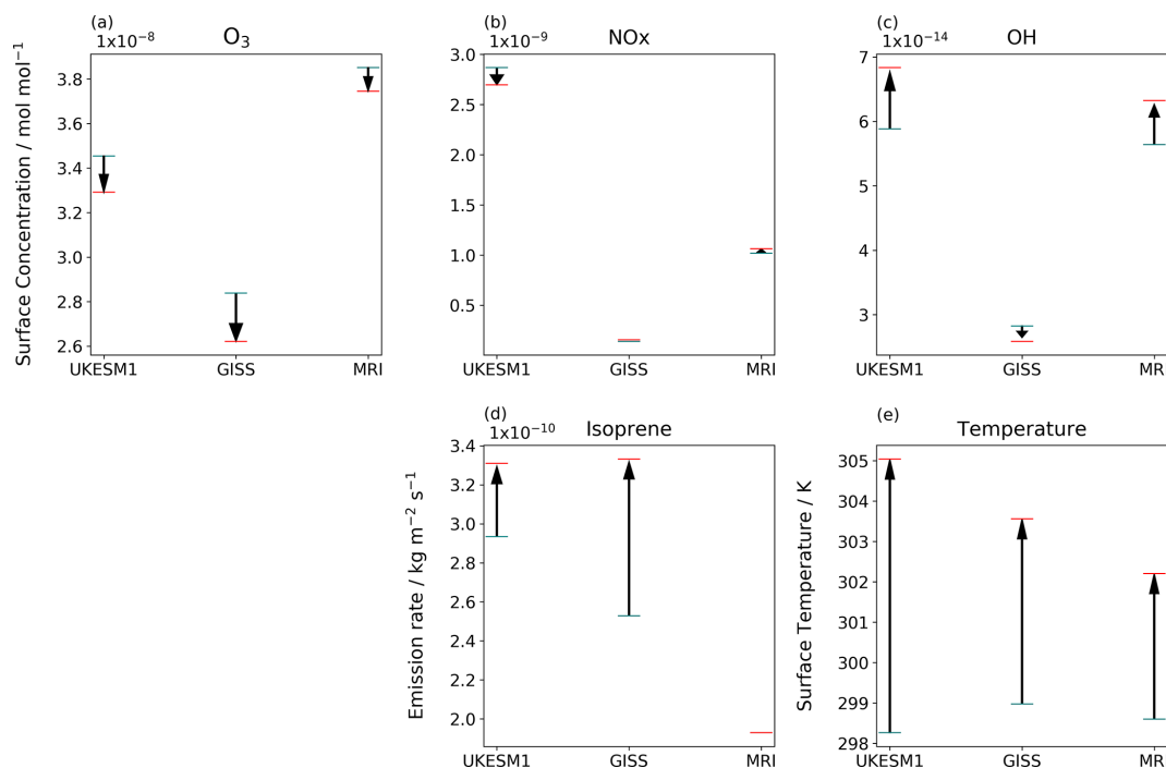
Figure 2. The change in surface concentration of (a) O 3 , (b) NO x and (c) OH, and the change in (d) isoprene emission rate and (e) surface temperature from experiment ssp370pdSST with no climate change (blue line) to experiment ssp370SST with climate change (red line) for the three climate models in this study. Variables have been averaged over the African and South American continents between 12° N–30° S for the period 2090–2100. The change due to climate change is significant at the 5 % level for all variables and models except isoprene in MRI (which is prescribed so does not change).
