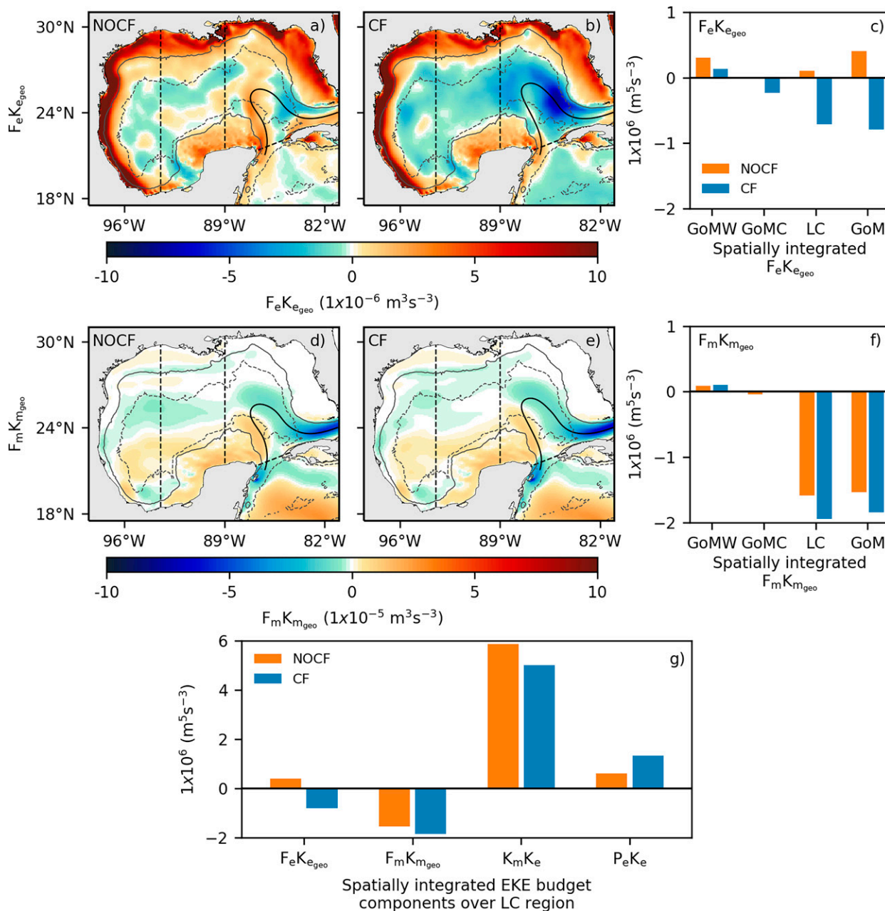
FIG. 6. (a),(b) Eddy and (d),(e) mean geostrophic wind work maps and (c),(f) spatially integrated values over regions for the NOCF and CF experiments for the period 1993–2016. The segmented lines delimit the east (LC), center (GoMC), and west (GoMW) regions. GoM refers to the whole Gulf of Mexico. The light gray contours refer to the depths of 200 m (continuous) and 2500 m (segmented). (g) Spatially integrated energy budget terms over the LC region.
