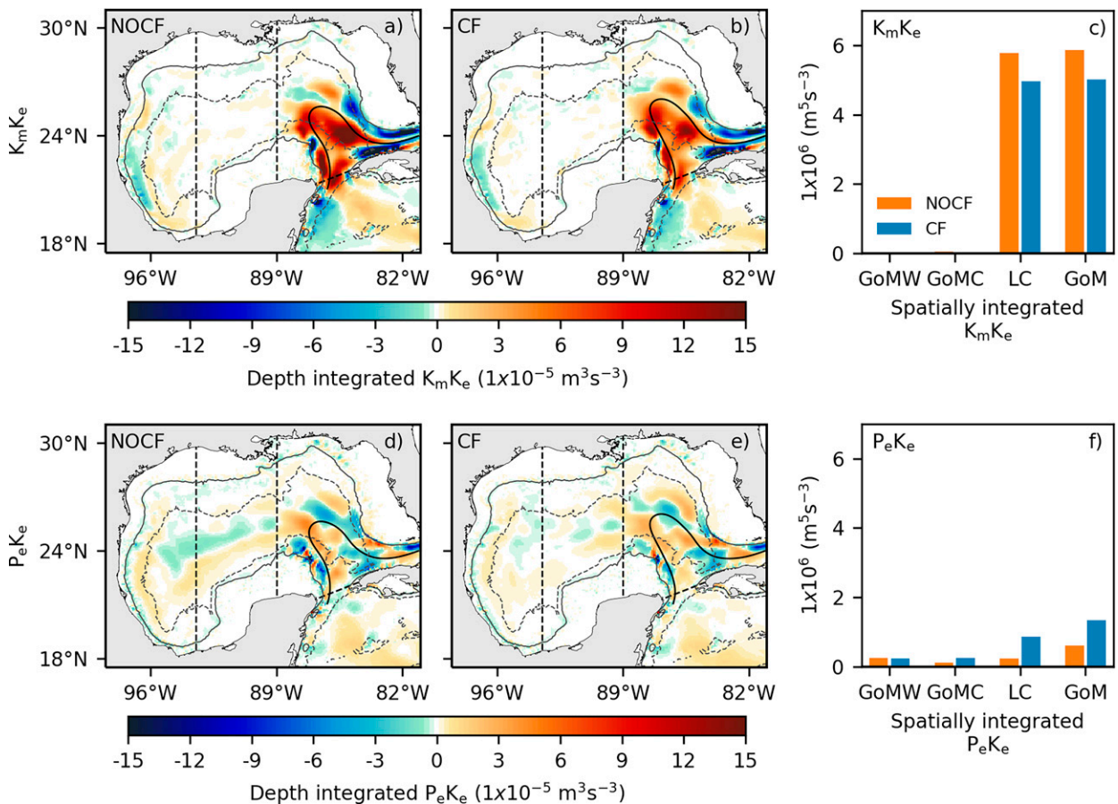
FIG. 5. (a),(b) Barotropic and (d),(e) baroclinic instabilities maps and (c),(f) spatially integrated values over regions for the NOCF and CF experiments for the period 1993–2016. The segmented lines delimit the east (LC), center (GoMC), and west (GoMW) regions. GoM refers to the whole Gulf of Mexico. The light gray contours refer to the depths of 200 m (continuous) and 2500 m (segmented).
