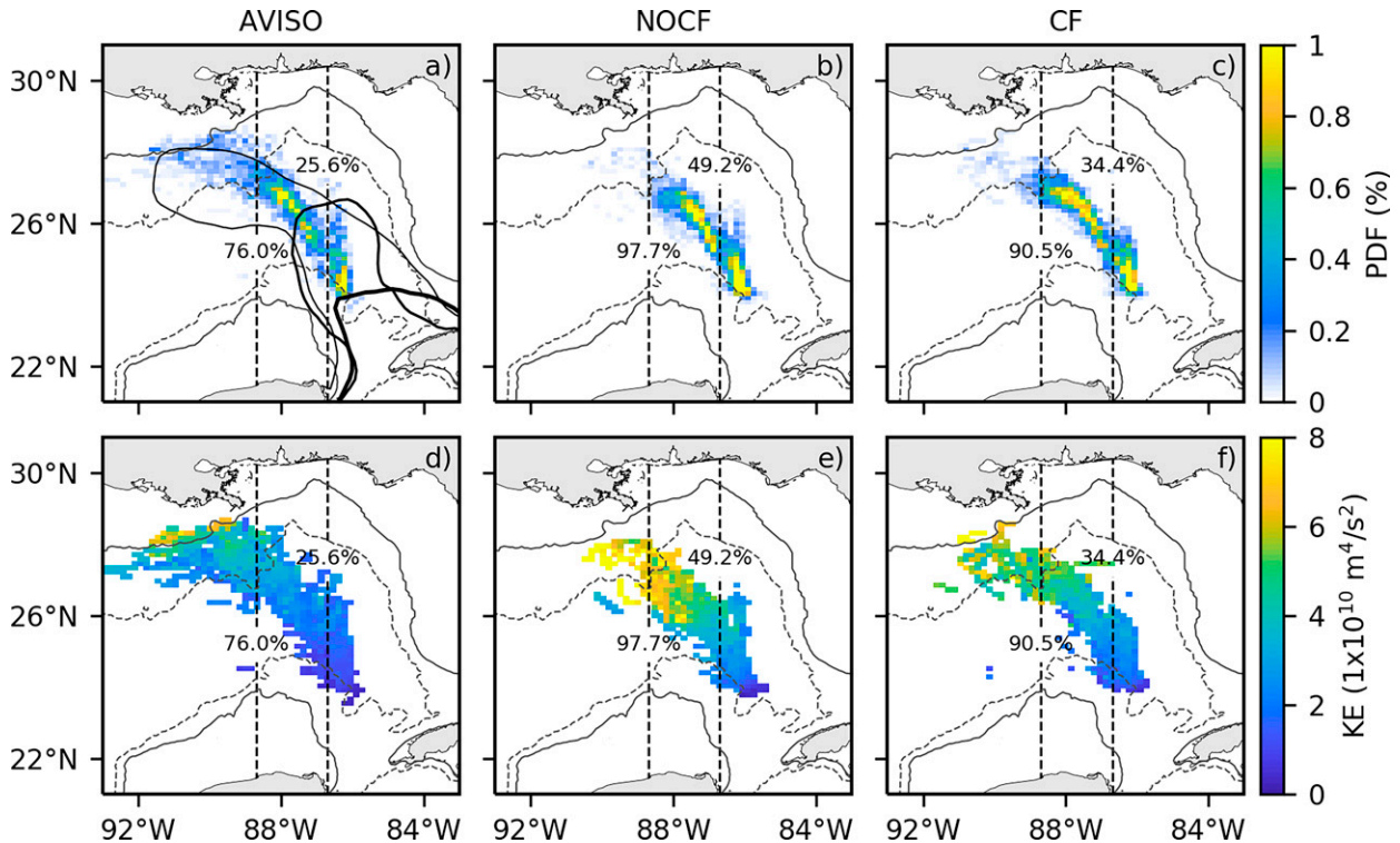
FIG. 7. Probability density functions related to the occurrence of LC maximum latitudes and longitudes for the period 1993–2016 for (a),(d) AVISO; (b),(e) NOCF; and (c),(f) CF and associated average of spatially integrated KE. The thick, medium-thick, and thin black contours represent examples of the retracted, canonical, and elongated LC forms, respectively. The light gray contours refer to the depths of 200 m (continuous) and 2500 m (segmented).
