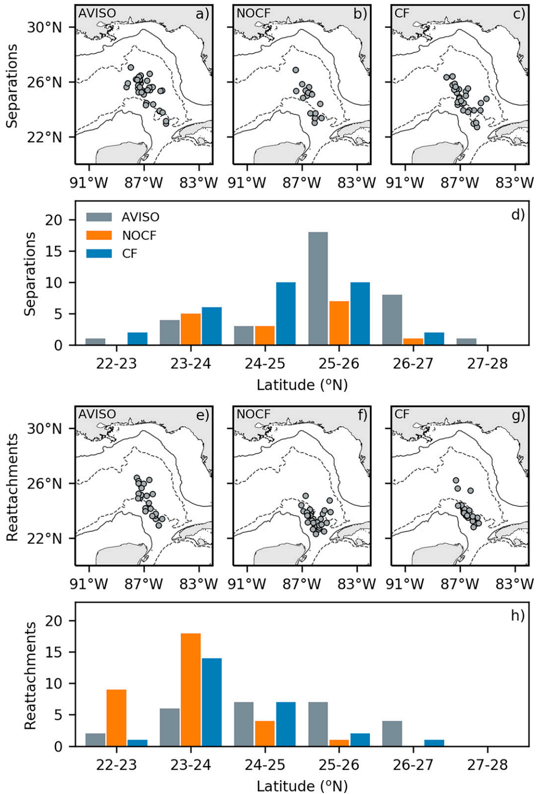
FIG. 10. LC most extended position (gray dots) after (a)–(c) separation and (e)–(g) reattachment events, for AVISO in (a) and (e), NOCF in (b) and (f), and CF in (c) and (g). The light gray contours refers to the depths of 200 m (continuous) and 2500 m (segmented). (d),(h) PDFs related to the latitude of the LC most extended position after separation and reattachment events are shown in (d) and (h).
