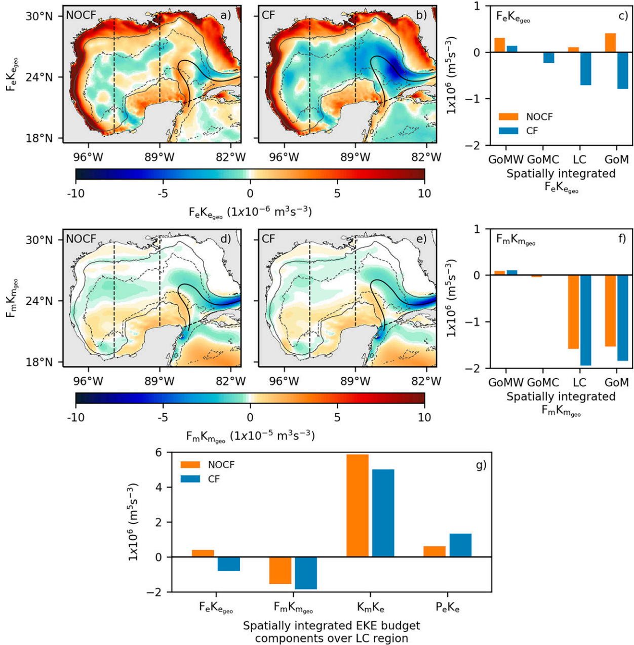
FIG. 6. (a),(b) Eddy and (d),(e) mean geostrophic wind work maps and (c),(f) spatially integrated values over regions for the NOCF and CF experiments for the period 1993–2016. The segmented lines delimit the east (LC), center (GoMC), and west (GoMW) regions. GoM refers to the whole Gulf of Mexico. The light gray contours refer to the depths of 200 m (continuous) and 2500 m (segmented). (g) Spatially integrated energy budget terms over the LC region.
