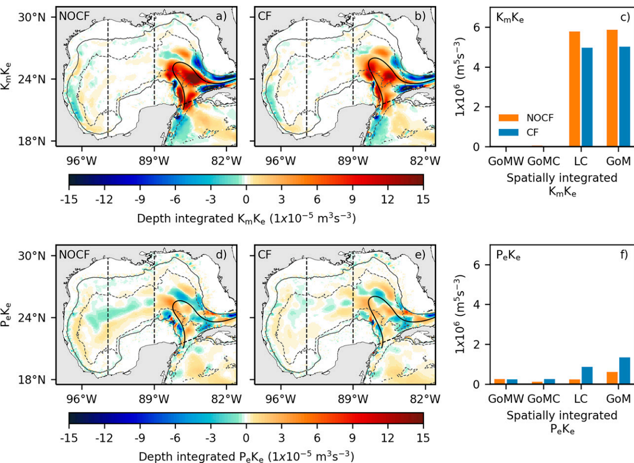
FIG. 5. (a),(b) Barotropic and (d),(e) baroclinic instabilities maps and (c),(f) spatially integrated values over regions for the NOCF and CF experiments for the period 1993–2016. The segmented lines delimit the east (LC), center (GoMC), and west (GoMW) regions. GoM refers to the whole Gulf of Mexico. The light gray contours refer to the depths of 200 m (continuous) and 2500 m (segmented).
