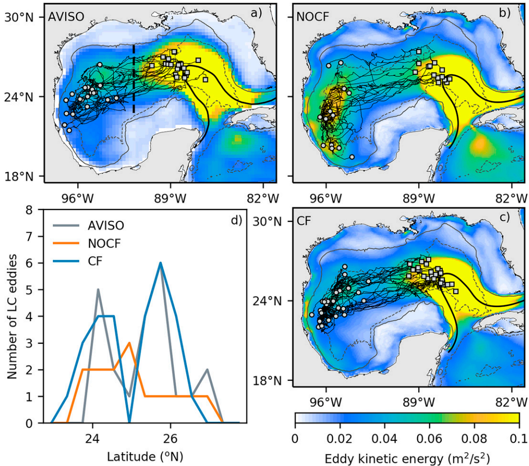
FIG. 9. Trajectories related to LC eddies with a lifetime longer than 200 days for (a) AVISO, (b) NOCF, and (c) CF. Gray squares represent the location of a LC eddy liberation, and gray circles the location where LC eddies are no longer detected. The color map refers to the corresponding EKE climatology. The 17-cm contours of the climatological sea surface height anomaly of AVISO and the numerical experiments are represented by the black line. The light gray contours refer to the depths of 200 m (continuous) and 2500 m (segmented). (d) Number of LC eddies that cross the segmented thick line shown in (a) as a function of the latitude.
