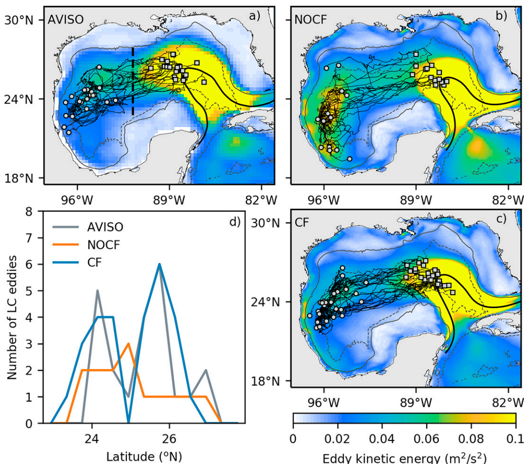
FIG. 9. Trajectories related to LC eddies with a lifetime longer than 200 days for (a) AVISO, (b) NOCF, and (c) CF. Gray squares represent the location of a LC eddy liberation, and gray circles the location where LC eddies are no longer detected. The color map refers to the corresponding EKE climatology. The 17-cm contours of the climatological sea surface height anomaly of AVISO and the numerical experiments are represented by the black line. The light gray contours refer to the depths of 200 m (continuous) and 2500 m (segmented). (d) Number of LC eddies that cross the segmented thick line shown in (a) as a function of the latitude.
