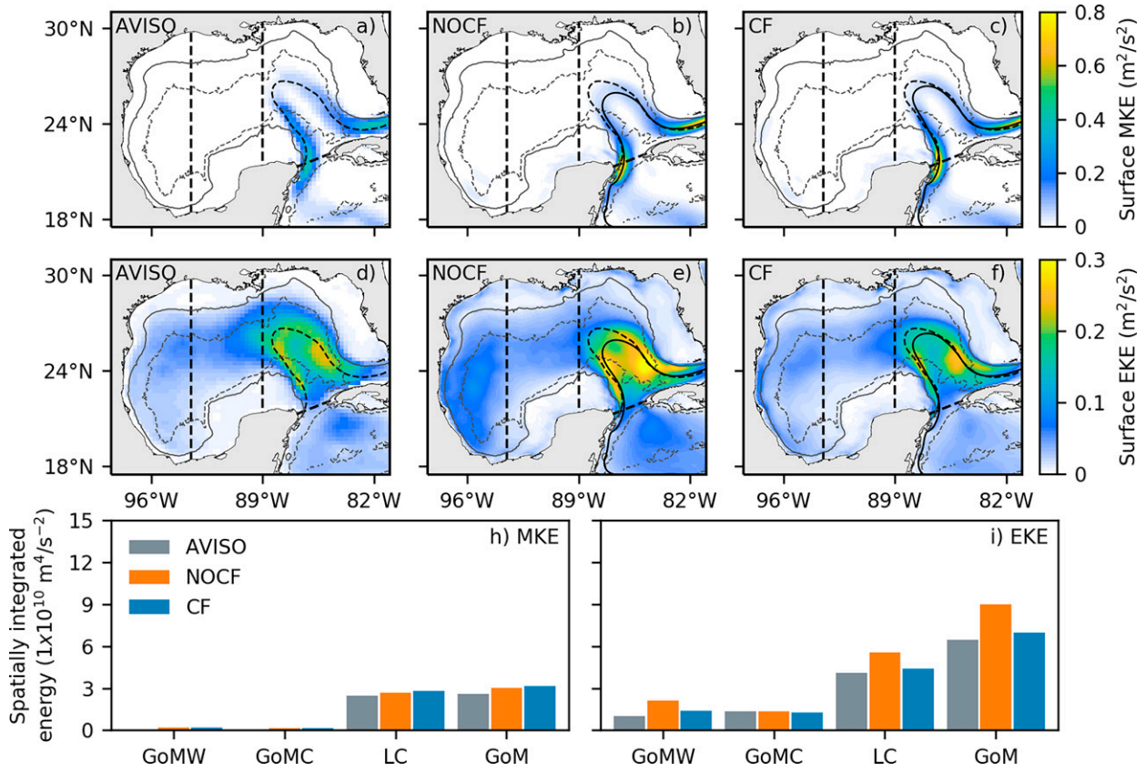
FIG. 2. (top) Surface mean kinetic energy and (middle) eddy kinetic energy climatologies (1993–2016) from (left) AVISO, (center) NOCF, and (right) CF. The 17-cm contours of the climatological sea surface height anomaly of AVISO and the numerical experiments are represented by the thin segmented line and the continuous line, respectively. The thick segmented lines delimit the east (LC), center (GoMC), and west (GoMW) regions. GoM refers to the whole Gulf of Mexico. The light gray contours refer to the depths of 200 m (continuous) and 2500 m (segmented). (bottom) Spatially integrated values over the regions.
