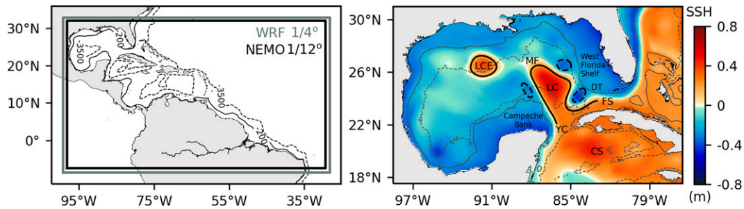
FIG. 1. (a) Intra-Americas Sea and (b) Gulf of Mexico. (a) The numerical domain for NEMO (WRF) is represented by the black (gray) box. The isobaths represent depths of 200 m (continuous lines) and 3500 m (dashed lines). (b) Main dynamical features of the GoM dynamics illustrated by a snapshot of the sea surface height anomaly. The continuous contours highlight the Loop Current (LC) and LC eddies. The dashed contours highlight the LC frontal eddies. YC is Yucatan Channel, FS is Florida Straits, DT is Dry Tortugas Islands, MF is Mississippi Fan, and CS is Caribbean Sea. The light gray contours refer to the depths of 200 m (continuous) and 2500 m (dashed).
