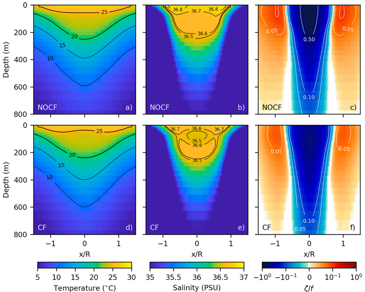
FIG. 11. LC eddy composite of (a),(d) temperature and (b),(e) salinity and (c),(f) the relative vorticity ( \zeta ) normalized with the Coriolis parameter ( f ) for (bottom) CF and (top) NOCF. Black and thick contours indicate thermoclines at 26- and 220-m depth. Normalized relative vorticity contours of 0.05, 0.1, and 0.5 are shown using white lines.
