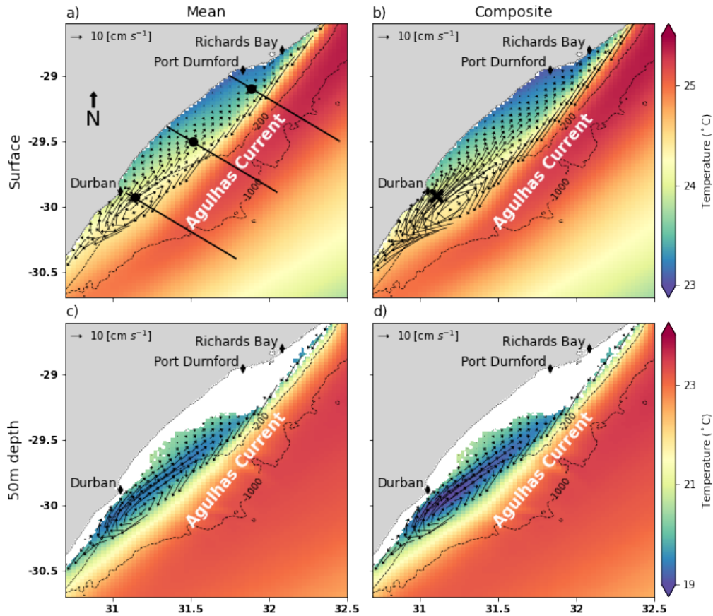
Figure 3: Maps of the modeled circulation and water temperature, derived from January 2005 to December 2014. In (a) and (b), the respective time-averaged and north-eastward composite of the surface circulation is presented. The north-eastward composites include north-eastward velocities that exceed 10 cm/s at 31.11°E and 29.93°S, marked by the black cross in (b). Similarly (c) and (d), respectively, represent the mean and composite circulation and the water temperature at 50 m depth. Velocities are masked for currents off the shelf which exceed 30 cm/s in (a) and (c) and 50 cm/s in (b) and (d). These regions that do not show the direction of the circulation are associated with a south-westerly flow. The offshore grey lines are the 200 m and 1000 m isobaths and the three transect lines in (a) are later used for further analysis. The black dots along the transects in (a) mark the points that have the most frequent north-eastward flow along each transect. It must be noted that the temperature scales are different for the surface plots and the plots at depth.
