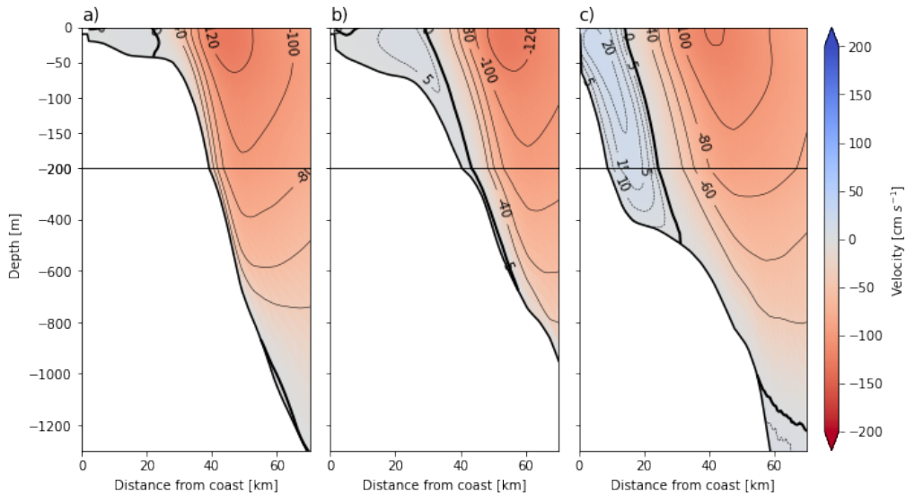
Figure 4: Modelled vertical sections of the 10 year mean current velocities derived across the transects and presented in Figure 3a. In (a), the northern transect is depicted, (b) shows the central transect and (c) represents the southern transect. The bold black lines are the transition lines between northward and southward velocities and the thinner solid black lines are the southward velocity contours, while the dotted thinner black lines are the northward velocity contours. A northward flow is positive and blue, while a southward flow is negative and marked with red.
