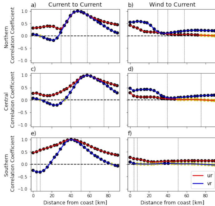
Figure 6: The Pearson correlation coefficient of the surface circulation at the Agulhas Current core and remaining points along the (a) northern, (c) central and (e) southern KZN Bight transects from Figure 3a, as well as the Pearson correlation coefficients of wind and surface currents along the (b) northern, (d) central and (f) southern transects. The red lines are the across-shore components ( u_r ) and the blue lines show along-shore components ( v_r ) of the correlations. The vertical black dotted lines indicate the location of the 50 m, 200 m and 1000 m isobaths. Black dots indicate correlations significant at the 95th percentile, while the remaining correlations are plotted using yellow dots.
