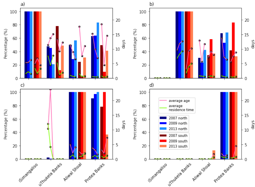
Figure 7: The average residence time (green lines) and the average age (pink lines) of virtual particles released in the (a) iSimangaliso, (b) uThukela Banks, (c) Aliwal Shoal and (d) Protea Banks Marine Protected Areas (MPAs). Within the KZN Bight, three northward surface flow events during 2007, 2009 and 2013 are indicated by the blue bars, while three southward surface flow events during the same years are indicated by red bars. The height of the bars indicates the percentage of virtual particles that enter each MPA, in each case.
