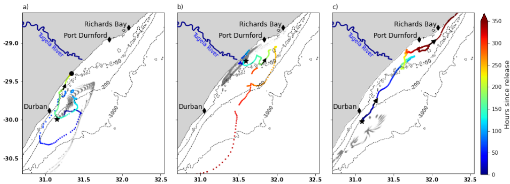
Figure 2: In colour are the trajectories of three NOAA designed drifters that were caught in a north-eastward shelf current in the KZN Bight. Release locations are indicated by black stars and when final locations are within the domain of the map, such as in panel a, they are marked by a black dot. Black arrows show the propagation direction at certain points along the trajectories. The colour of the trajectory is the time since release, measured in hours. Grey dots are the trajectories of 100 virtual particles released in the CROCO model, per panel, at the same location and for the same time period as the drifters.
