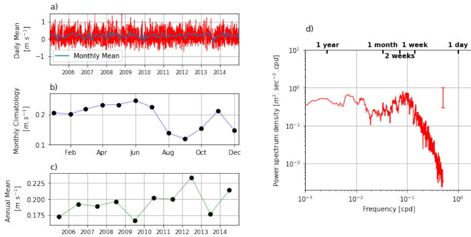
Figure 5: Time-series of the (a) daily and monthly means, (b) monthly climatology and (c) annual means of the 10-year model surface circulation in the KZN Bight at the point with the strongest mean north-eastward shelf flow marked in Figure 3b (31.11°E, 29.92°S). Currents are rotated -50^\circ to display the alongshore circulation and the monthly means are superimposed on the daily mean figure. In (d), the power spectrum density of the total signal of the surface currents is presented, using the multitaper method. The error bar represents the 95% confidence interval of the signal and the frequency unit is cycles per day (cpd).
