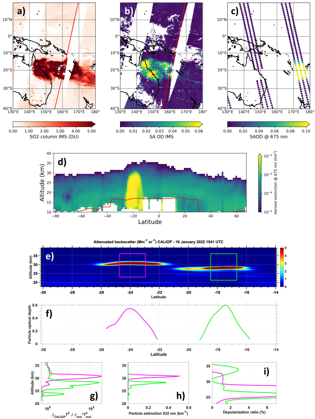
Fig. 2 The physicochemical properties of the early HT plume. IMS/IASI SO 2 ( a ) and sulfate-specific AOD ( b ) observations for 16th January at 23:07 UTC. a, b the red line is CALIOP track for the same day at 15:41 UTC. OMPS-LP integrated SAOD ( c ) and vertical aerosol extinction profile (central detector, d ) for 16th January at 2:03 and 3:27 UTC. d the red line is tropopause height. Attenuated CALIOP backscatter at 532 nm ( e ), and integrated in-plume AOD ( f ), corrected transmission ( g ) extinction ( h ) and depolarisation ( i ) in the two identified plumes sections (pink and green squares). The CALIOP track of e-i is the one identified in a and b . Due to the time mismatch between CALIOP and IASI orbits, the CALIOP track actually crossed both the eastern part of the aerosol plume in a, b (lower plume at 27 km) and the western part (upper plume at 30 km) which has already reached Australia in the display.
