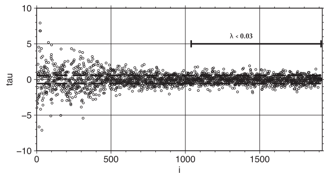
Figure 2. The set of 1947 transformed data \tau_i for a cluster of mantle earthquakes in the Aleutians. There are 820 \tau_i for which \lambda_i < 0.03 , and their distribution allows us to estimate the error distribution of the delay times for this cluster. The dashed lines indicate the \sigma_e estimate of 0.58 s from the distribution of this subset of \tau_i .
