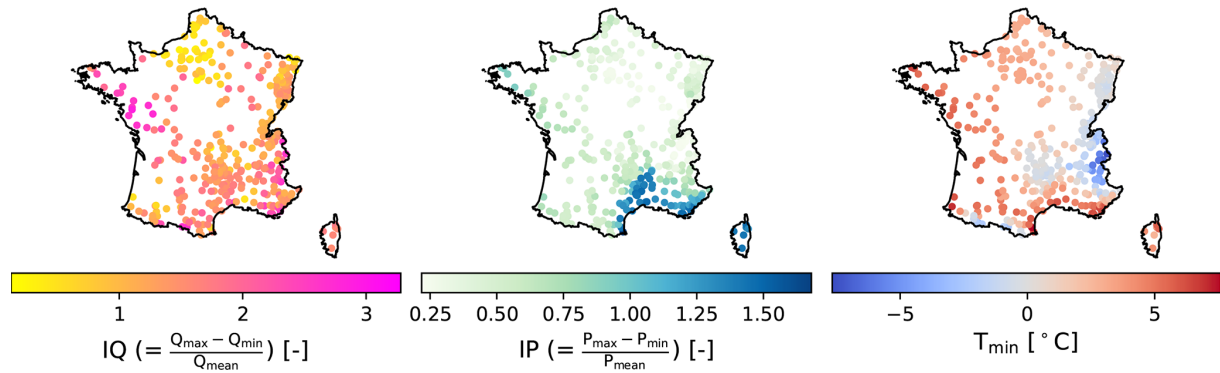
Figure 1. Spatial variation in the three indices used for hydrologic catchment classification: IQ, IP, and T_{\min} . Each catchment in the sample is shown as a point.
