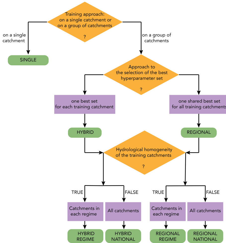
Figure 8. Conceptual flowchart of how SINGLE, REGIONAL, and HYBRID LSTM models and their submodels (green rounded rectangles) are built based on three decision criteria (orange rhombuses): the training approach, the approach to the selection of the best hyperparameters, and the training catchments.
