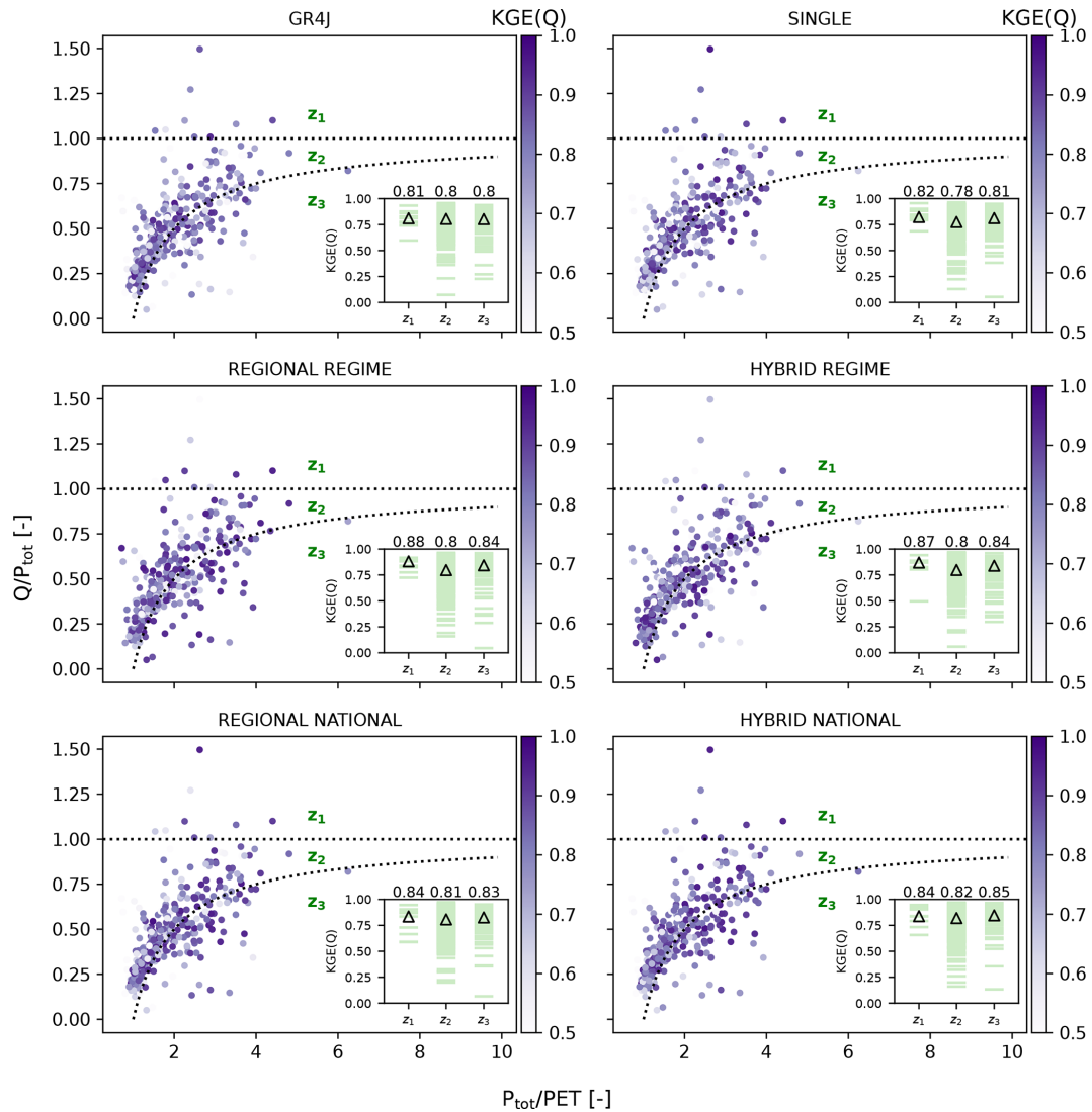
Figure 12. Variation in KGE scores with respect to the runoff ratio ( \frac{Q}{P_{tot}} ) and wetness index ( \frac{P_{tot}}{PET} ) for the GR4J and LSTM models. Scores lower than 0.5 are shown in the same tone as the lower extreme of the colour bar. The inset plot within each panel shows the KGE scores of the catchments located in each of the z_1 (above the horizontal water limit line), z_2 (between the horizontal and curved lines), and z_3 (below the curved line) zones. The ( \Delta ) symbol and numbers in the inset plots represent the median KGE scores of the three zones. The KGE scores correspond to the test data, with the exception of the first 2 years, which constitute the warm-up period in GR4J and for which there are no outputs.
