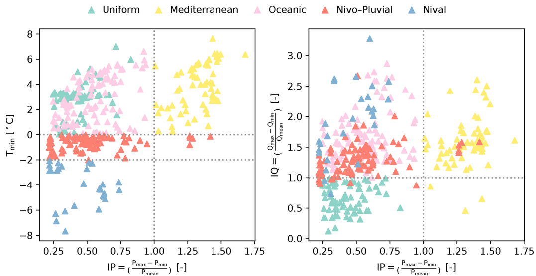
Figure 2. Classification of the catchments into five hydrologic regimes based on five conditions built on T_{min} , IP, and IQ. In order of priority, we first evaluate two T_{min} conditions: T_{min} < -2 and T_{min} < 0 . For catchments not satisfying either of these two conditions, we then check if IP > 1 . If this condition is also unsatisfied, the IQ > 1 condition is evaluated. Each point represents a catchment, and its colour indicates its regime.
