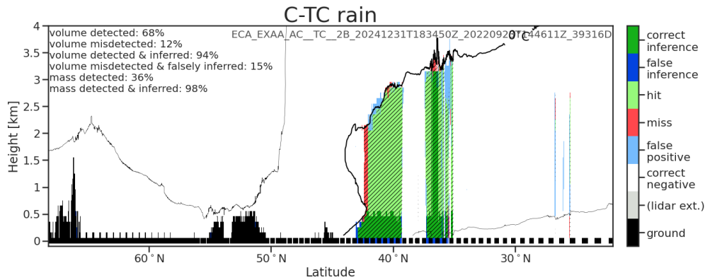
Figure 13. An intercomparison of AC-TC detection of rain for the Halifax scene. The volume fraction is calculated from the fraction of pixels detected compared to those containing any rain in the GEM model after interpolation to the JSG (hatched areas). The mass fraction is based on the mass of rain from the GEM model. The total fractions in AC-TC include the inferred presence of rain that cannot be detected directly by the instrument but may be inferred, such as in regions of radar surface clutter contiguous with rain or where CPR is extinguished in deep convection. Atmospheric temperature contours from the model are overlaid. Grey shading indicates where each instrument is extinguished.
