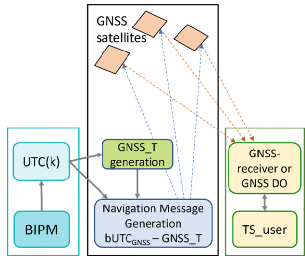
Figure 1. Timing elements involved in relating UTC and TS\_user via GNSS. The central block contains the elements under the responsibility of a GNSS provider, to the left the elements accessed from the metrological community and to the right the user part.
