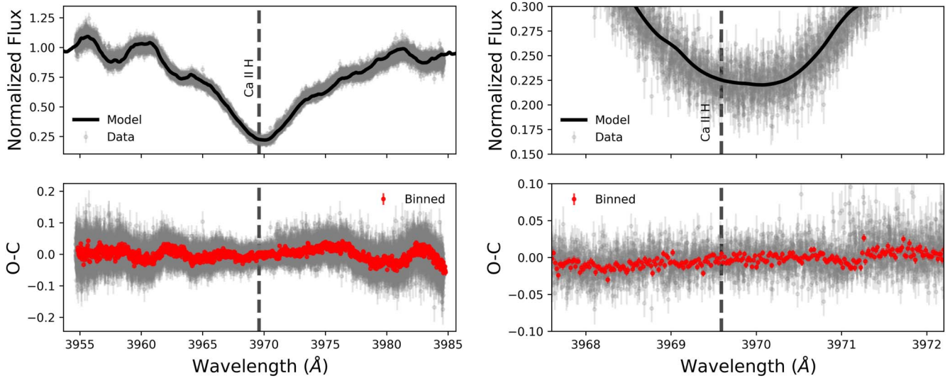
Figure 4. Data from LCOGT NRES spectra of the primary star HIP 5319 A compared to a PHOENIX model spectrum for an F5IV star surrounding the Ca II H line at its vacuum wavelength \lambda = 3969.5 \text{ \AA} . The model spectrum has been broadened by 100 \text{ km s}^{-1} to match the best-fit v \sin(i) value for the Ca II H line from the LCOGT spectra. (Left top) Model spectra plotted over data from the 12 LCOGT spectra between \lambda = 3955\text{--}3985 \text{ \AA} . (Left bottom) The O–C (Observed–Calculated) plot showing the residuals between measured data and model. Gray points are the residuals from each of the 12 spectra, while the red points are rebinned to the original NRES spectral resolution. (Right) The same data and residuals between \lambda = 3968\text{--}3972 \text{ \AA} . In both cases it can be clearly seen that there is no excess flux beyond the 1% level in the spectrum at any point near the Ca H line.
