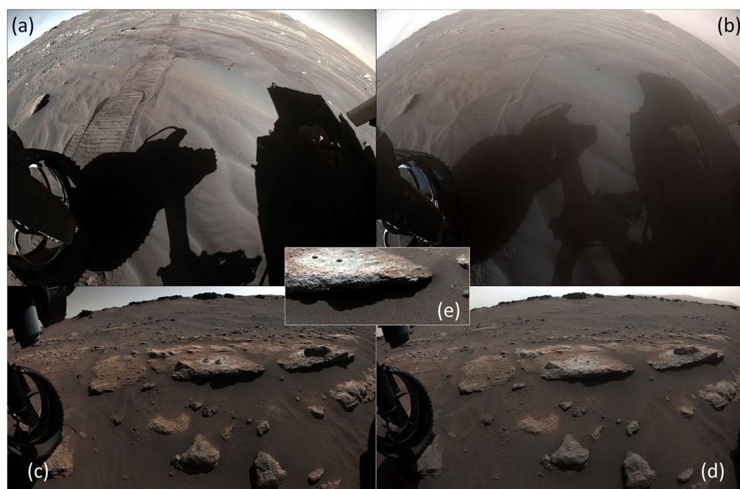
Figure 3. Changes immediately around the rover as seen in Rear (a), sol 286; (b), sol 316) and Front Hazcam (c), sol 311; (d), sol 315; (e), sol 322). (See Movie S3 and Movie S4.).
