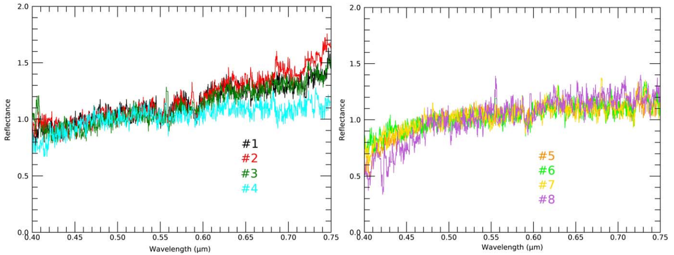
Figure 1. All the spectra observed in the 2021 apparition from TNG. Spectra 1–7 were observed on the night of February 15, while spectrum 8 was observed on February 23. All spectra are normalized at 0.55 \mu\text{m} .
