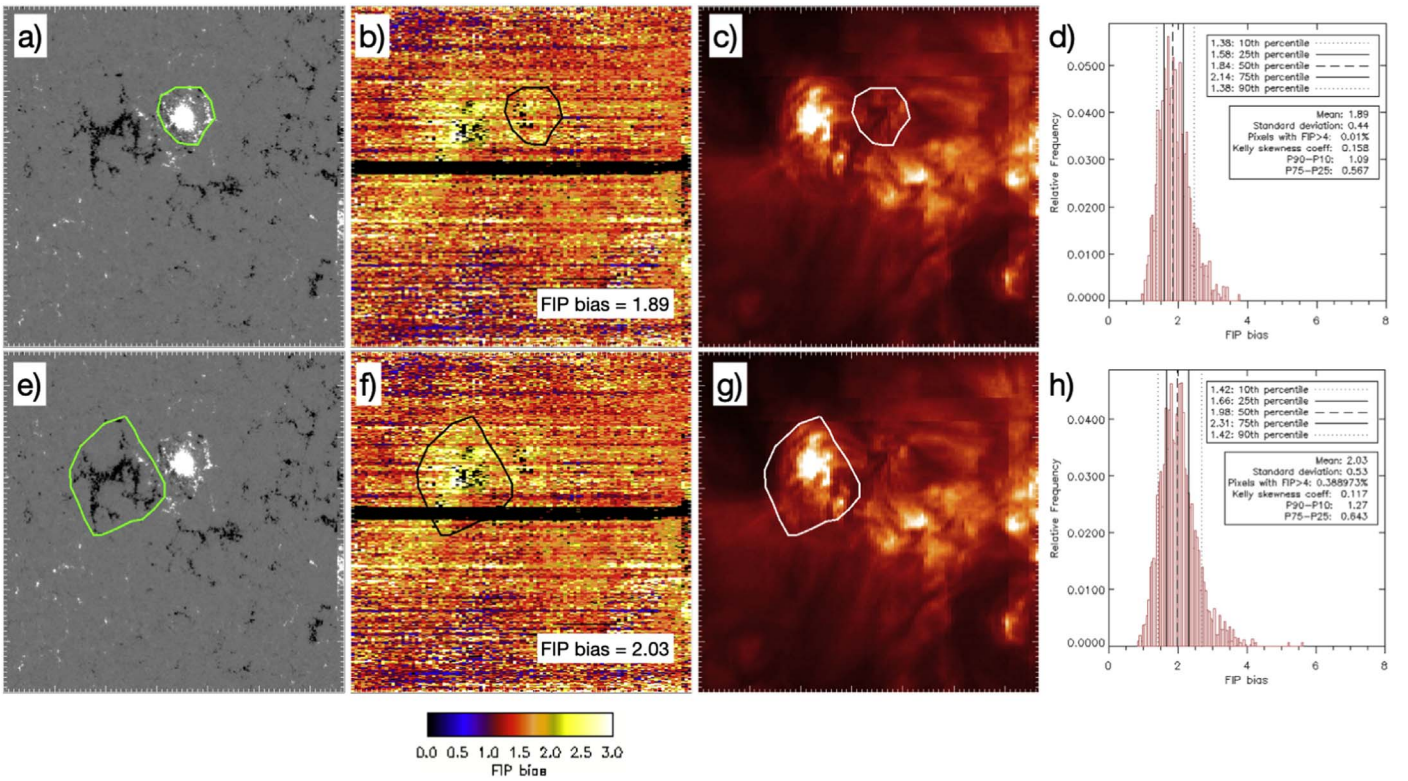
Figure 6. Case study of the median FIP bias in the leading (top) vs. following (bottom) polarities of R1 (2013 January). The maps show: (a), (e) HMI LOS photospheric magnetic field strength; (b), (f) Hinode/EIS FIP bias; (c), (g) Hinode/EIS Fe XIII 202.04 Å intensity; and (d), (h) histograms of the FIP bias within the contours shown in green, black, and white on the other panels. The values in the two boxes show the median FIP bias value in the defined contour.
