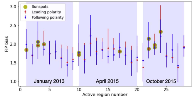
Figure 5. FIP bias in leading (red) vs. following (blue) polarities. The x-axis indicates the active region R code (1–28) used within the data set, as defined in Figure 1. The vertical bars indicate the FIP bias spread, i.e., the 25th and 75th percentile of the distribution in each region. The 50th percentile is highlighted with a star. Active regions that still have a sunspot are highlighted with a yellow dot.
