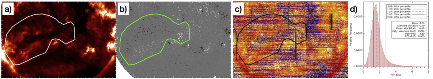
Figure 7. Case study of R11 (2015 April): (a) Hinode/EIS Fe XIII 202.04 Å intensity, (b) HMI line-of-sight magnetic field strength, (c) Hinode EIS FIP bias, and (d) FIP bias distribution within the active region contour.
