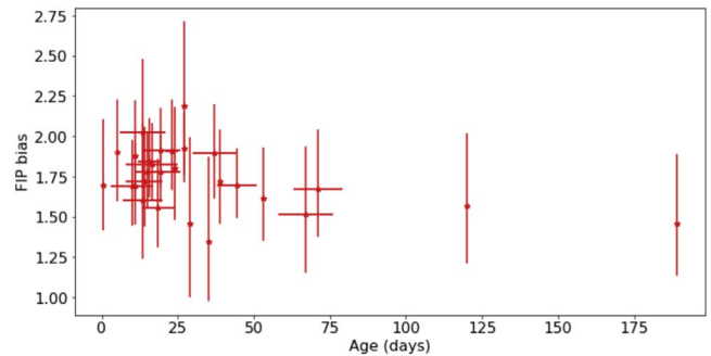
Figure 3. FIP bias variation with active region age. The vertical bars indicate the FIP bias spread, i.e., the 25th and 75th percentile of the distribution in each region. The 50th percentile is highlighted with a star. The error bar associated with the age measurement corresponds to the minimum and maximum age for that region, in case there was no observation available at the time and location of its emergence.
