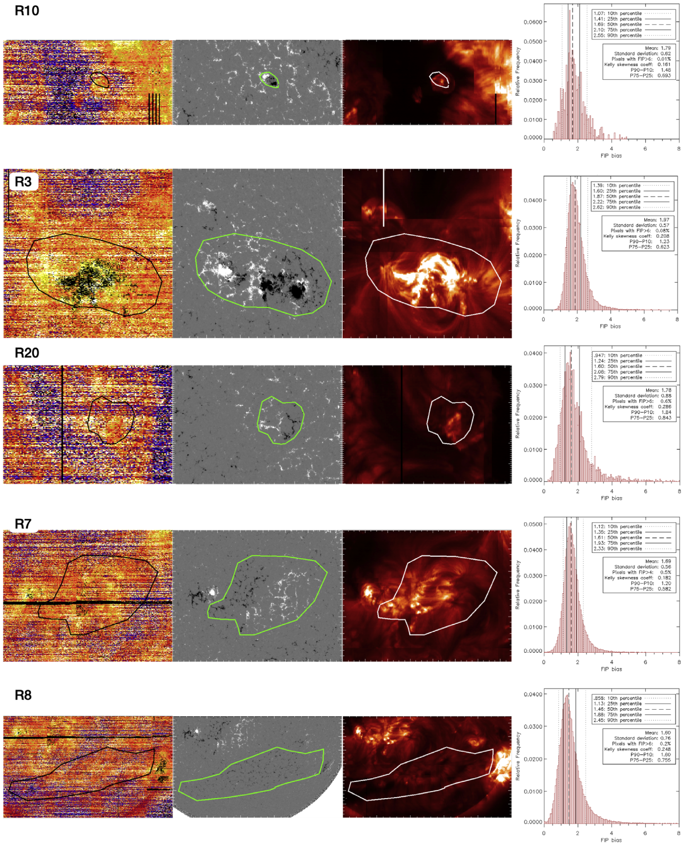
Figure 8. Examples of FIP bias distributions in the selected active region contours for each of the active region categories listed in Table 3. From left to right: Hinode EIS FIP bias, HMI line of sight magnetic field strength, XIII 202.04 Å intensity, and FIP bias distribution within the active region contour (shown in black, green, and white, respectively). The complete figure set (28 elements) is available in the online journal.
