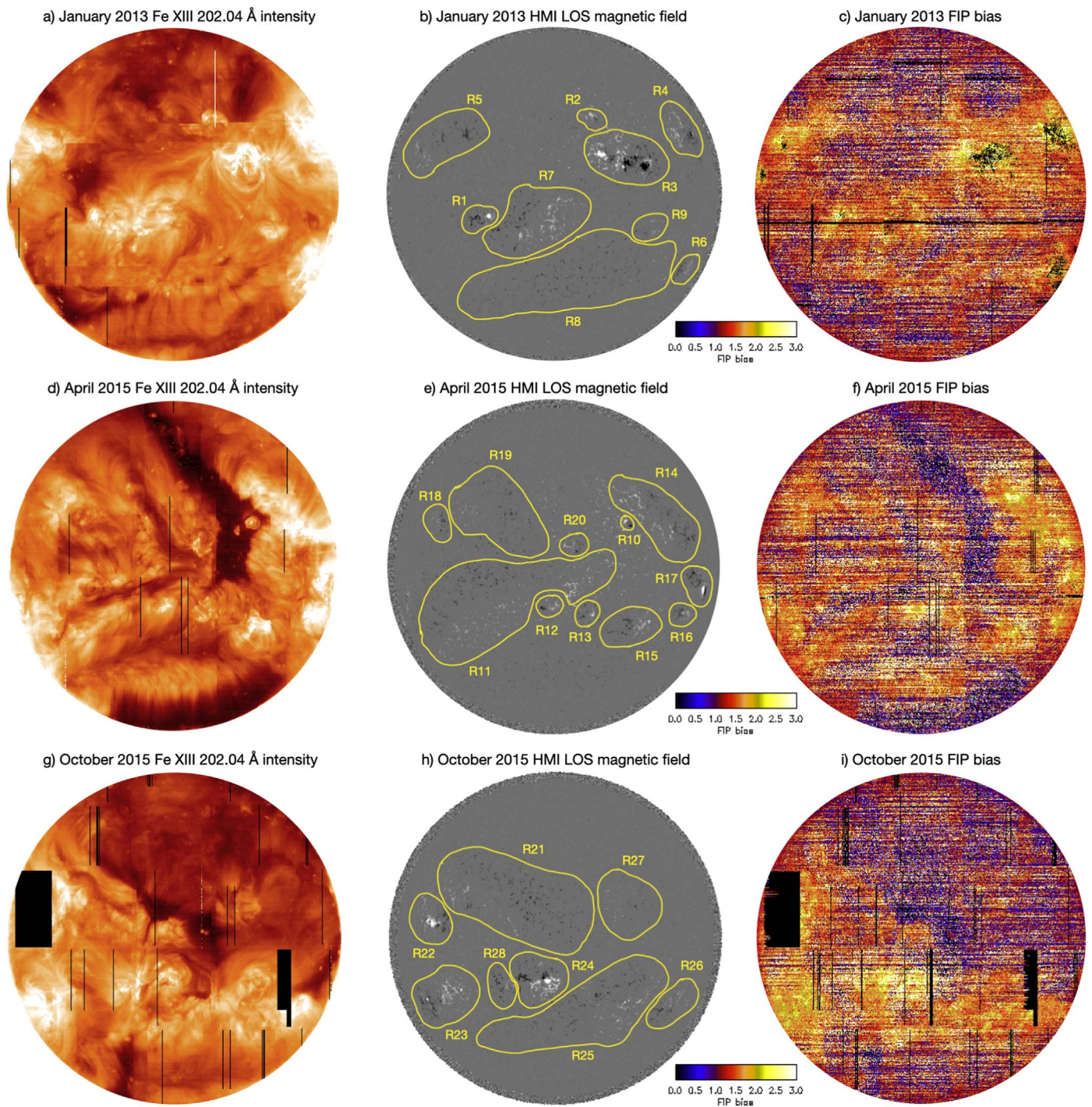
Figure 1. Full Sun maps constructed from: (a), (d), (g) Hinode/EIS Fe XIII 202.04 Å intensity; (b), (e), (h) HMI line of sight photospheric magnetic field strength with overlaid active region contours (in yellow); (c), (f), (i) Hinode/EIS FIP bias. The black boxes present in the FIP bias and Fe XIII 202.04 Å intensity maps represent gaps in the EIS data. Individual active region contours overlaid on Hinode/EIS Fe XIII 202.04 Å intensity, HMI line-of-sight photospheric magnetic field strength, and Hinode/EIS FIP bias maps are shown in the Appendix .
