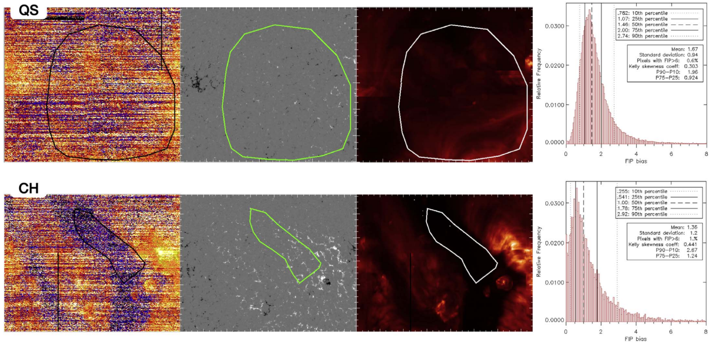
Figure 9. FIP bias distributions in selected representative examples of quiet Sun (QS) and coronal hole (CH). From left to right: Hinode EIS FIP bias, HMI line-of-sight magnetic field strength, Hinode/EIS Fe XIII 202.04 Å intensity, and FIP bias distribution within the selected contour (shown in black, green, and white, respectively).
