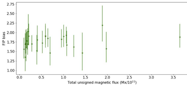
Figure 2. FIP bias variation with total unsigned magnetic flux of the active region. The vertical bars indicate the FIP bias spread, i.e., the 25th and 75th percentile of the distribution in each region. The 50th percentile is highlighted with a star.
