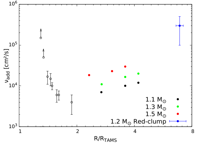
Fig. 12. Evolution of the efficiency of AM redistribution, parametrised by the additional viscosity \nu_{\text{add}} , as a function of the radius normalised to the radius at the end of the MS. Black dots with R/R_{\text{TAMS}} < 2 correspond to subgiants studied by Deheuvels et al. (2020) and Eggenberger et al. (2019b). The other symbols correspond to red giants in the phase of hydrogen-shell burning with different initial masses and finally to the estimate for red clump stars based on a 1.2 M_{\odot} model.
