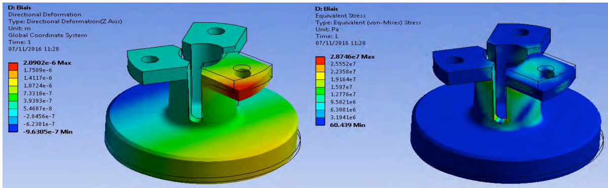
Figure 6. Analysis of the thermal sensitivity of the M2 mirror to planarity variations at the interface feet/support plate (to define its required regulation) of some 50 \mu rad.
