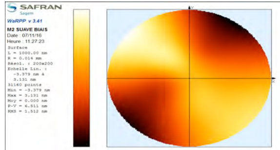
Figure 7. Opto-thermo-mechanical analysis of the secondary mirror of SUAVE on its nominal orbit and solar flux lightning configuration was carried and showed that, even with 50 \mu rad deformation at feet/plate interface, the peak-to-peak surface error of the mirror stays in within prescriptions, < 1 nm (deformations of a few nm are observed, up to 6 nm, but less than 0.6 nm after refocus).
