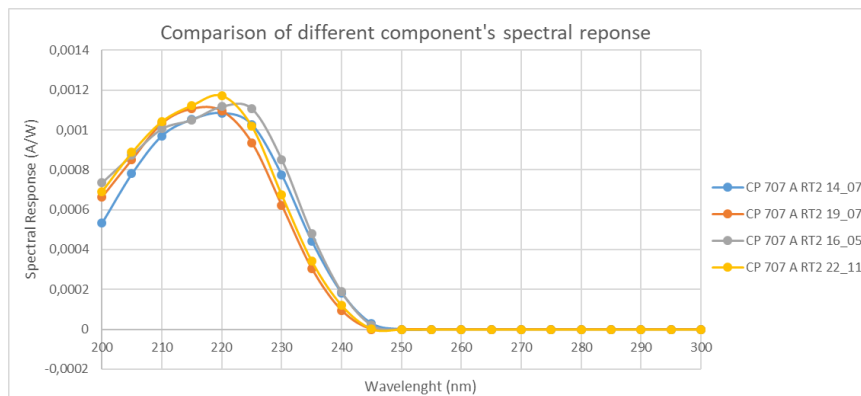
Fig. 1. Group of 4 \beta -Ga 2 O 3 DEVINS components selected for the Nanosatellite INSPIRE-Sat 7 and presenting an excellent rejection (solar blind for \lambda > 250 nm), centering (peak between 215-220 nm) and FWHM (~35 nm).
