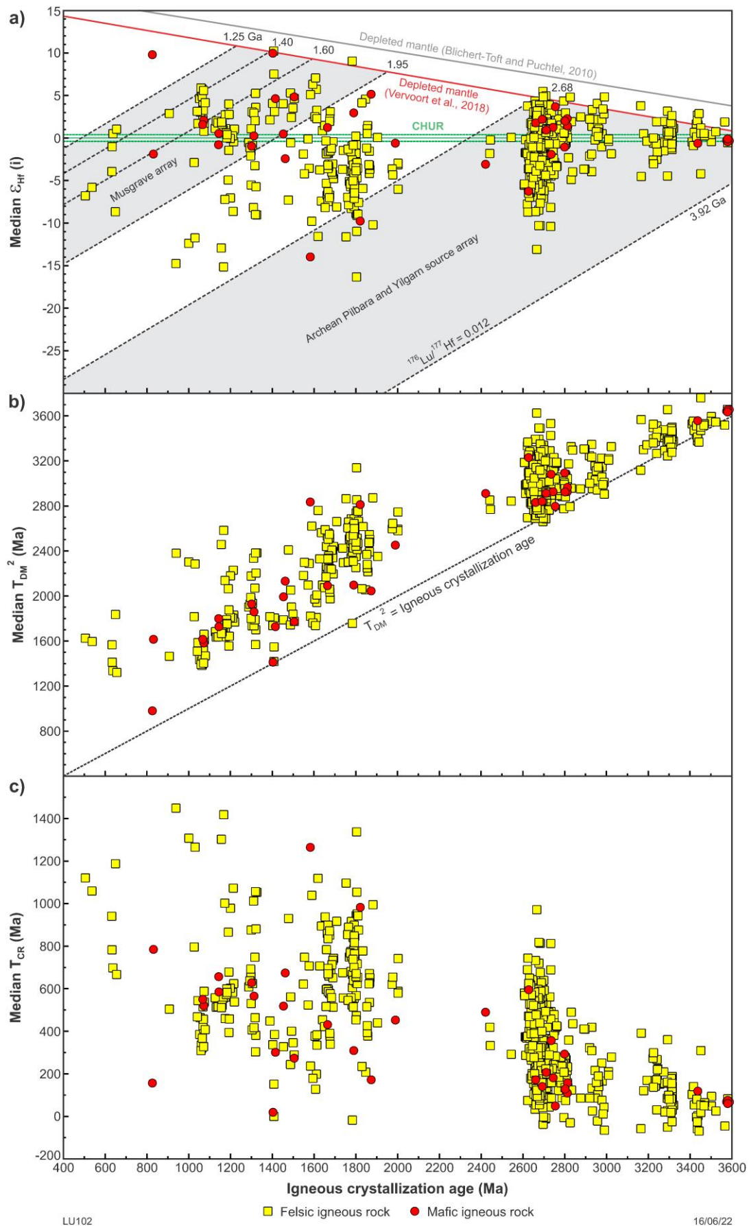
Figure 4. Values of median \epsilon_{\text{Hf}(i)} (a), T_{\text{DM}}^2 (b), and T_{\text{CR}} (c) vs igneous crystallization age for zircon samples of felsic and mafic igneous rocks in Western Australia. Samples on or close to the depleted mantle lines in (a) or the T_{\text{DM}}^2 = \text{igneous crystallization age} line in (b) indicate juvenile mantle input. The Musgrave array and Archean Pilbara and Yilgarn source array in (a) is from Lu et al. (2022b)
