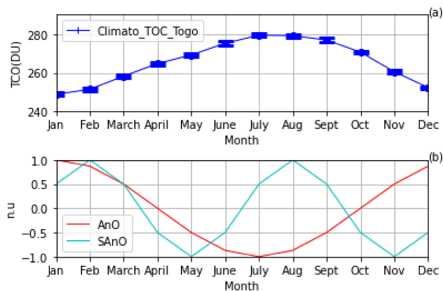
Figure 2. Climatology of the TOC (a) and the estimated proxies corresponding to the AnO and SAnO (Equation (1)) to simulate the climatology of the TOC (b) in the DU above Togo. The TOC is in the DU while the AnO and SAnO are in non-units (n.u.).
