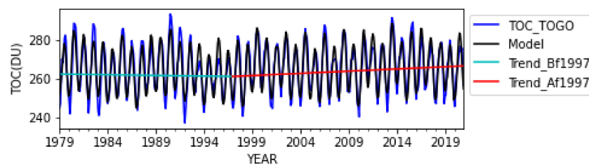
Figure 5. Evolution of the monthly average ozone over Togo observed by MSR-2, simulated by the MLR model, and the trends estimated by the model before and after 1997.
